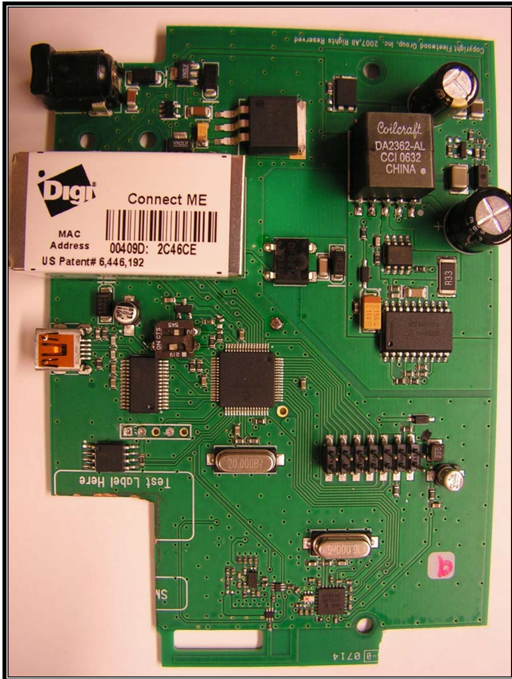
Photograph 222: PCB Top
