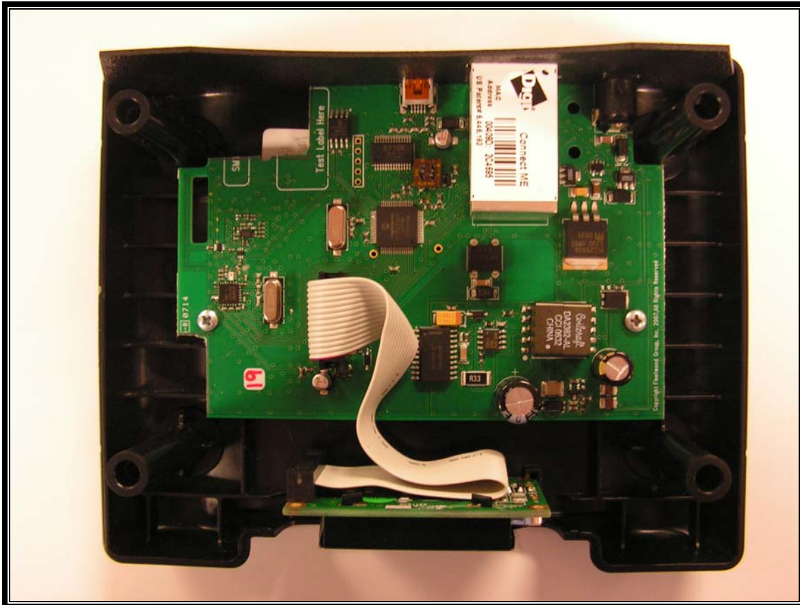
Photograph 21: Internal View
