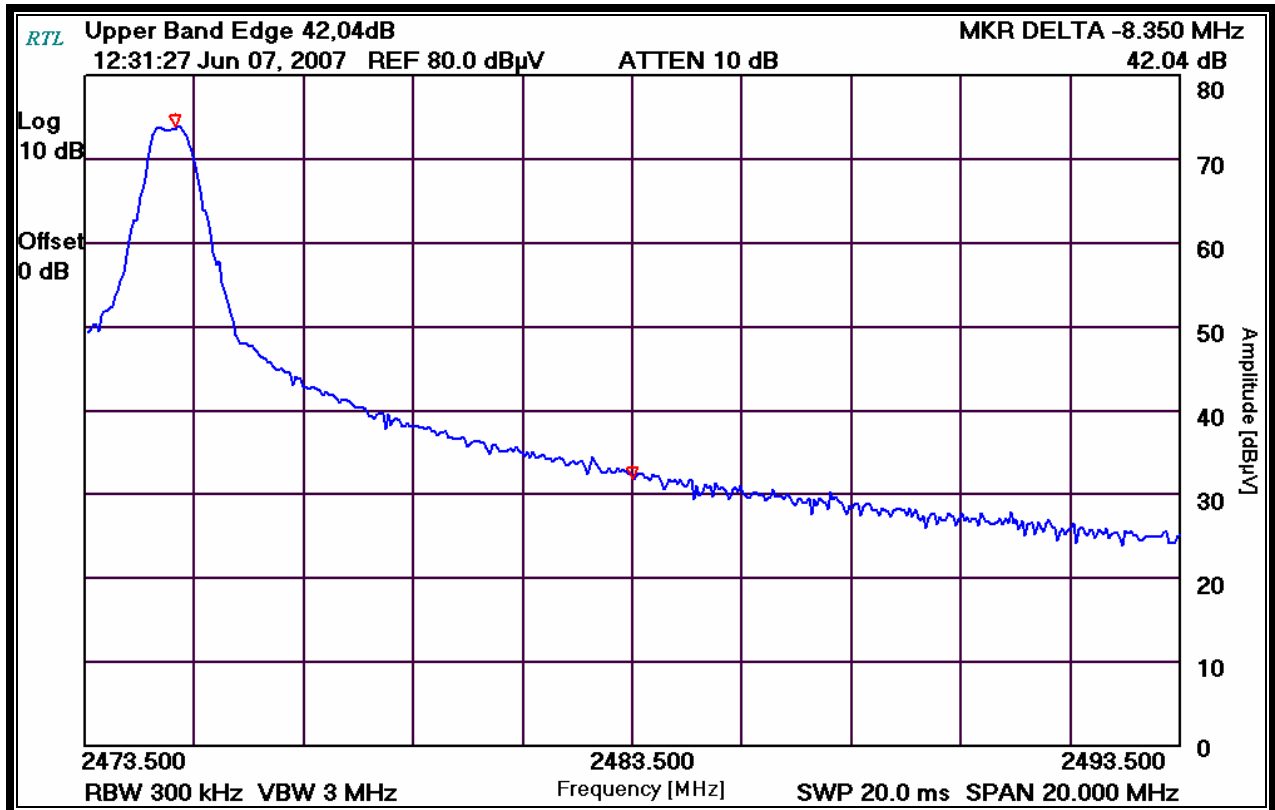
Plot 5-3: Conducted Upper Band Edge – Fixed High Channel Operation
