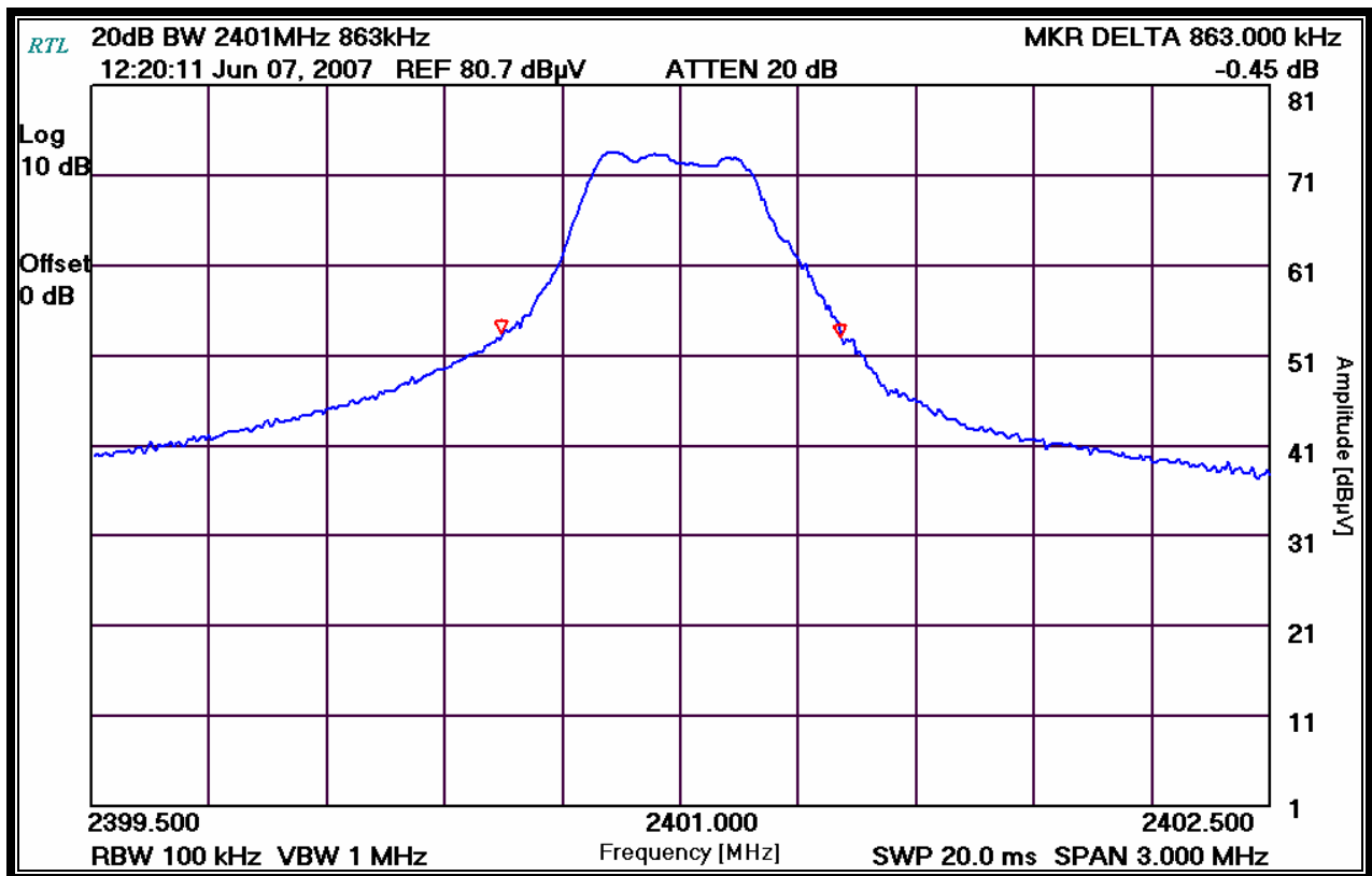
Plot 7-1: 20 dB Bandwidth Channel 1
