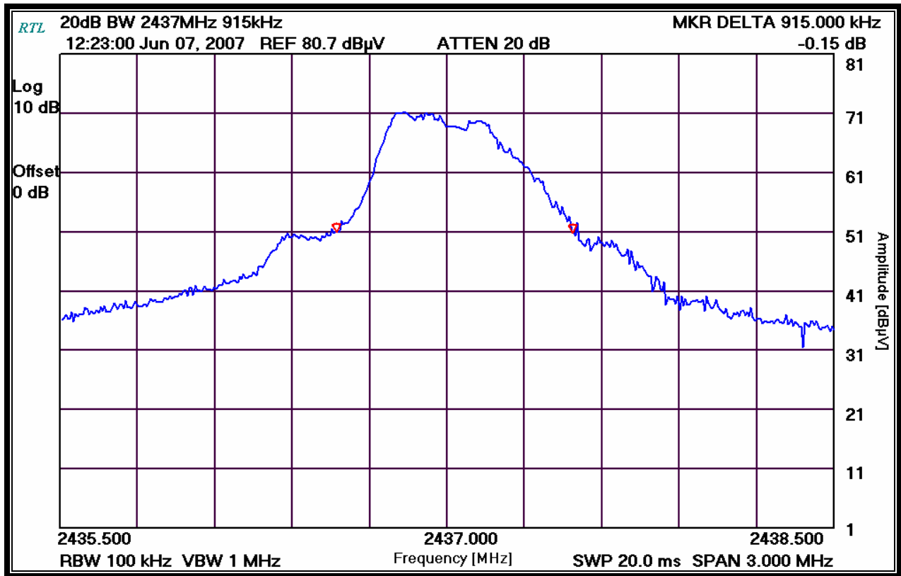
Plot 7-2: 20 dB Bandwidth Channel 37
