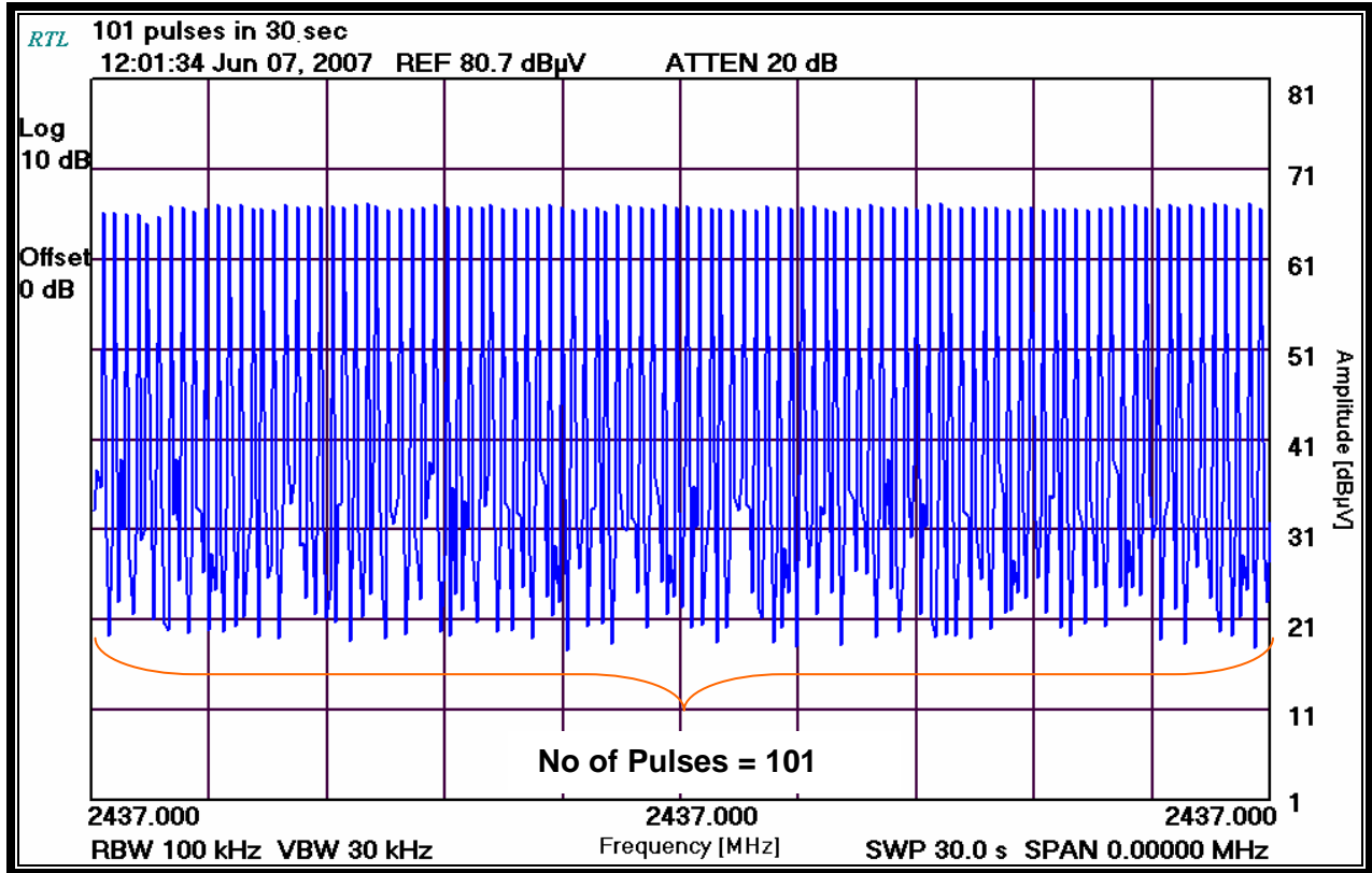
Plot 8-4: Time of Occupancy (Dwell Time 30 Second Sweep)
