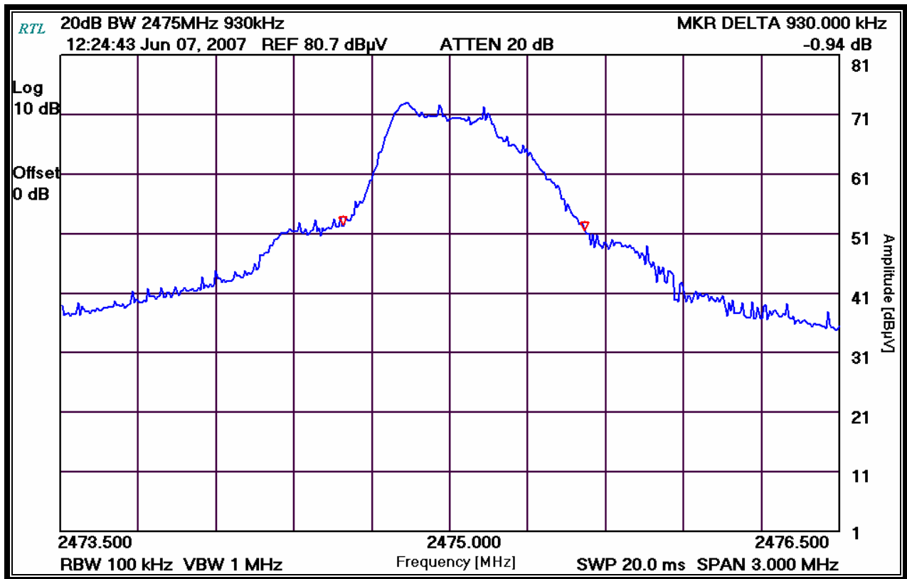
Plot 7-3: 20 dB Bandwidth Channel 75
