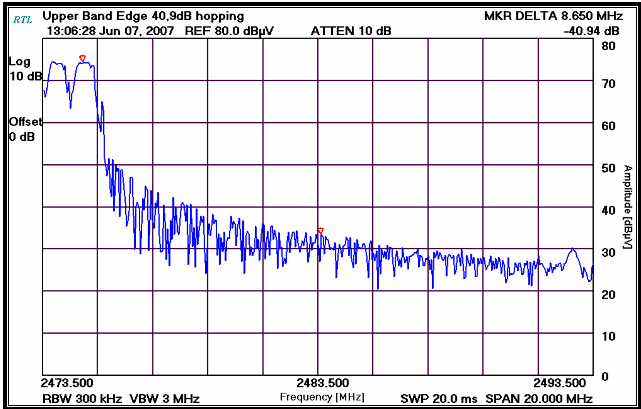
Plot 5-4: Conducted Upper Band Edge – Hopping
