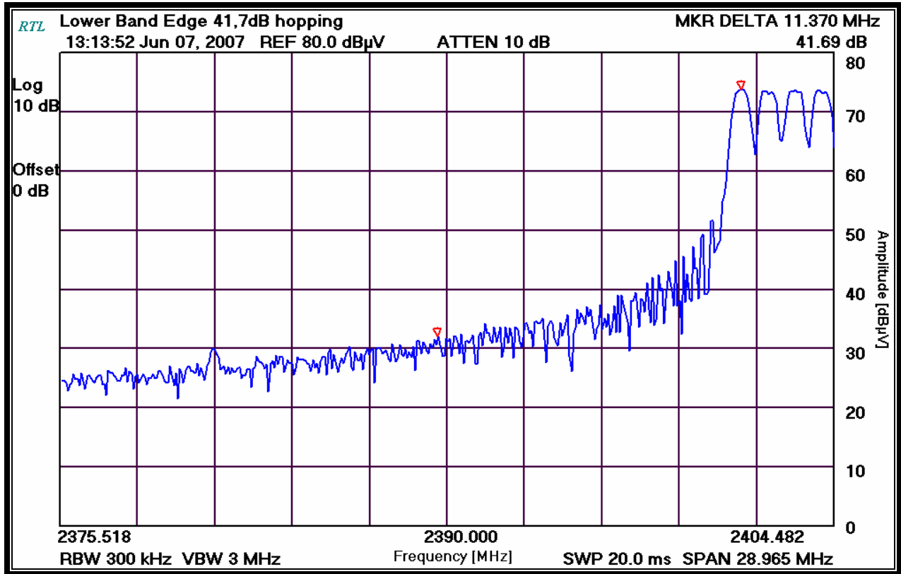
Plot 5-2: Conducted Lower Band Edge – Hopping
