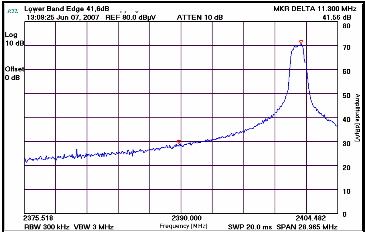
Plot 5-1: Conducted Lower Band Edge – Fixed Low Channel Operation
