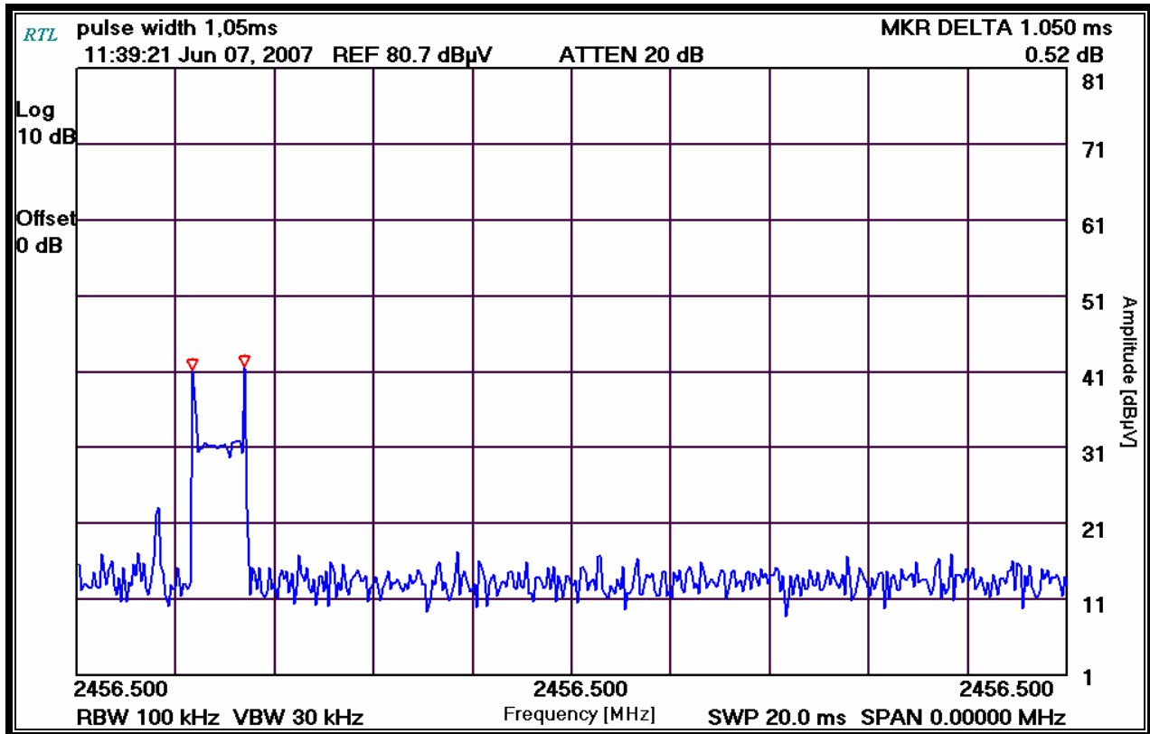
Plot 8-3: Time of Occupancy (Dwell Time)
