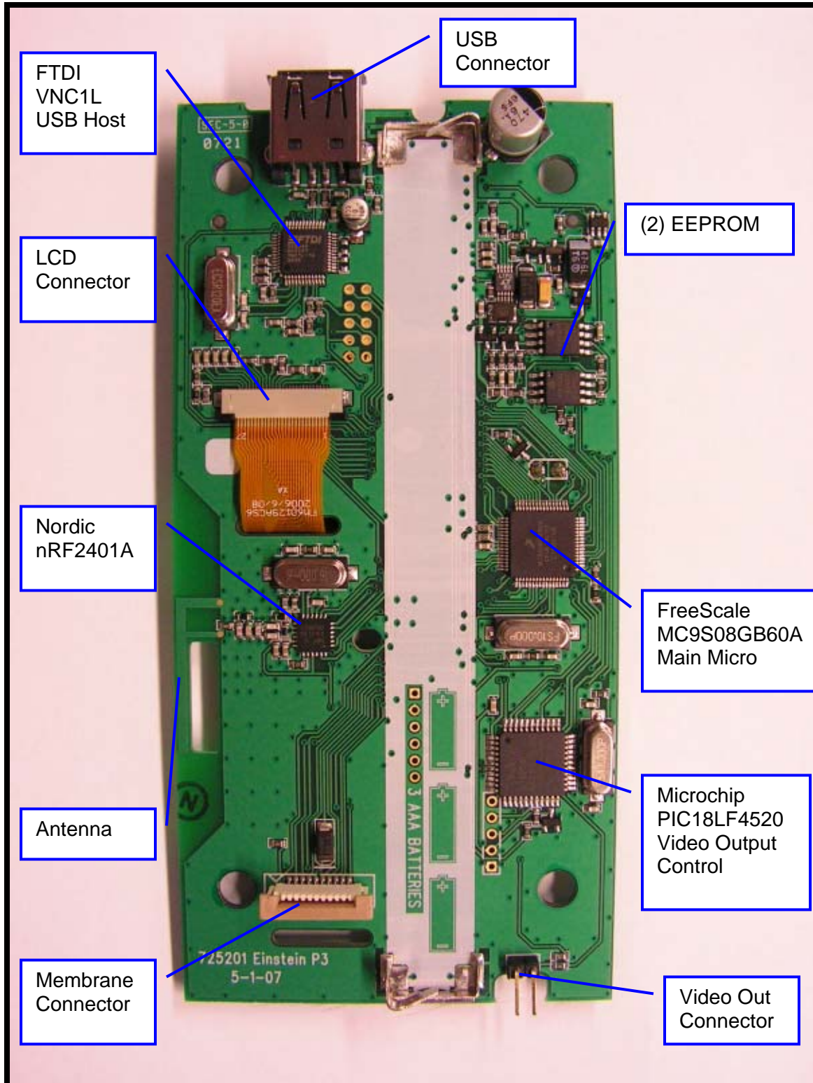
Photograph 12: Bottom of PCB
