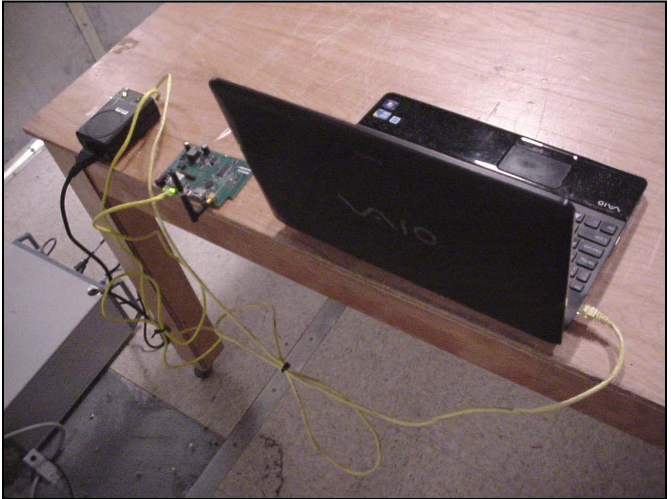
Photograph 6: Conducted Testing – Back View (Power Over Ethernet)
