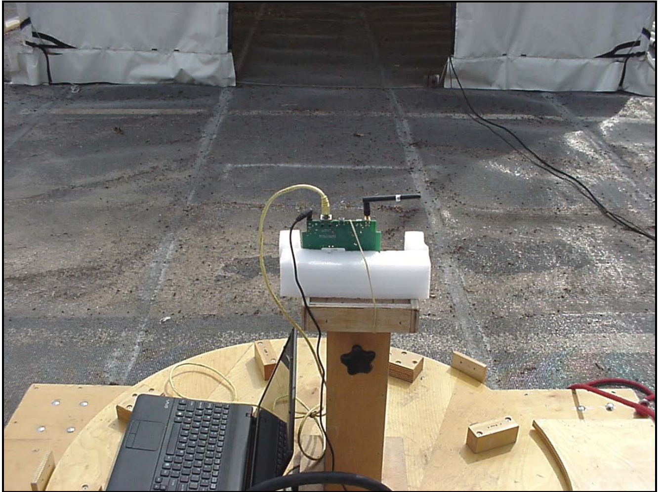
Photograph 4: Radiated Testing – Back View
