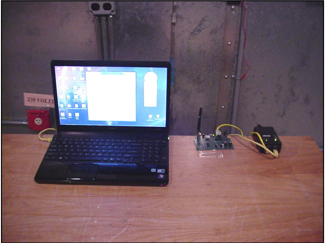
Photograph 5: Conducted Testing – Front View (Power Over Ethernet)
