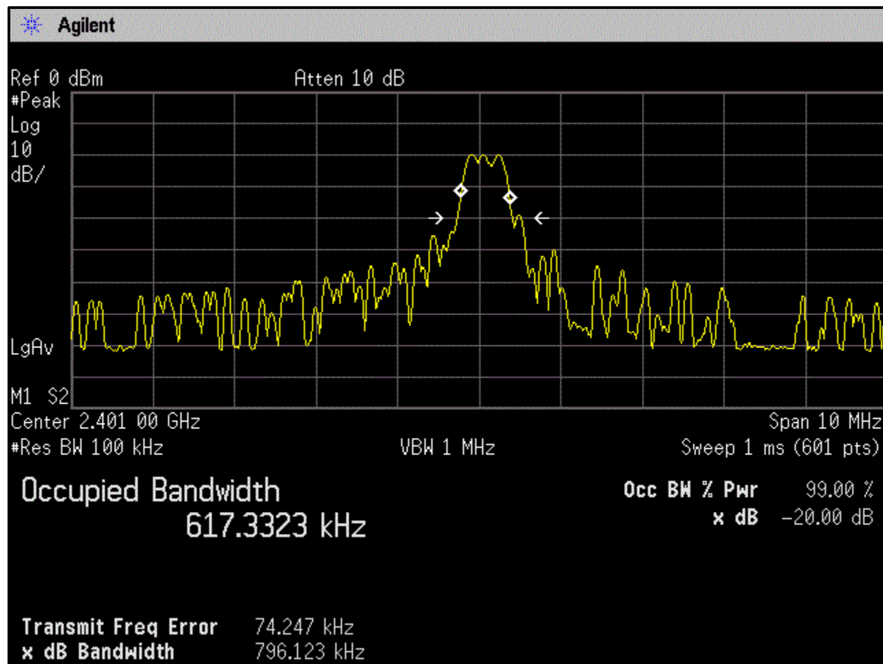
Plot 6-1: 20 dB Bandwidth Channel 1
