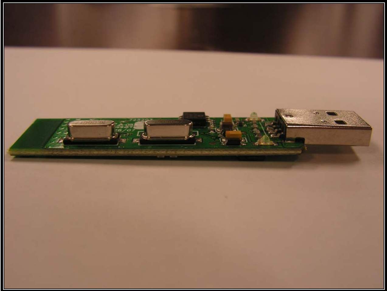
Photograph 7: USB240D Left Side
