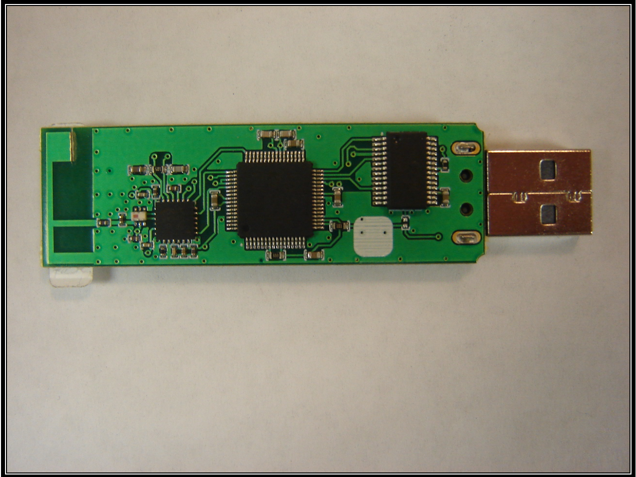
Photograph 6: USB240D Back
