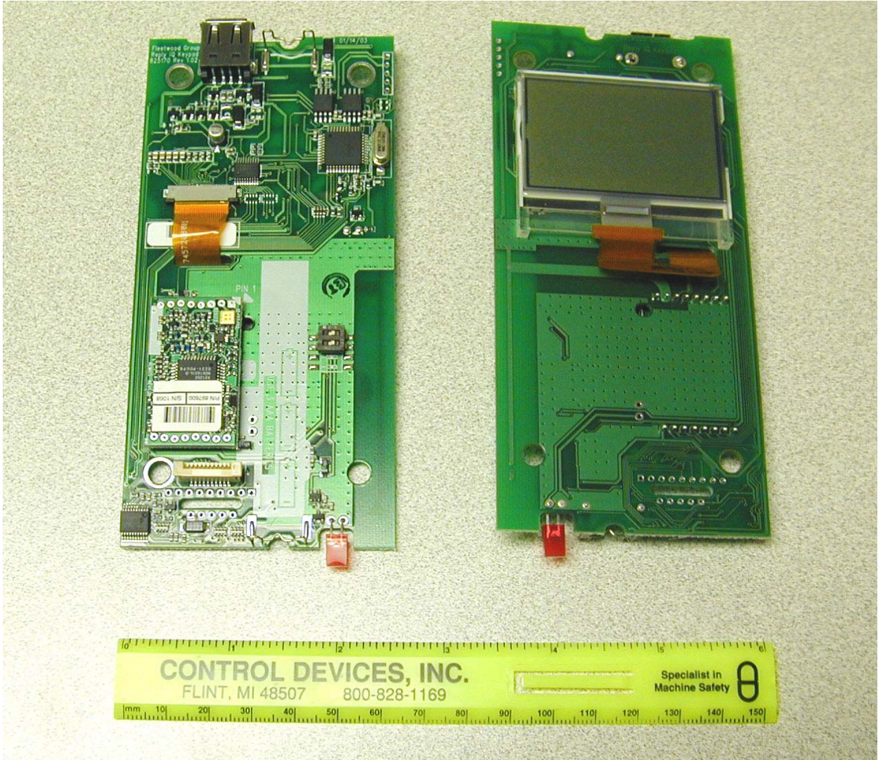
Keypad Circuit Board
