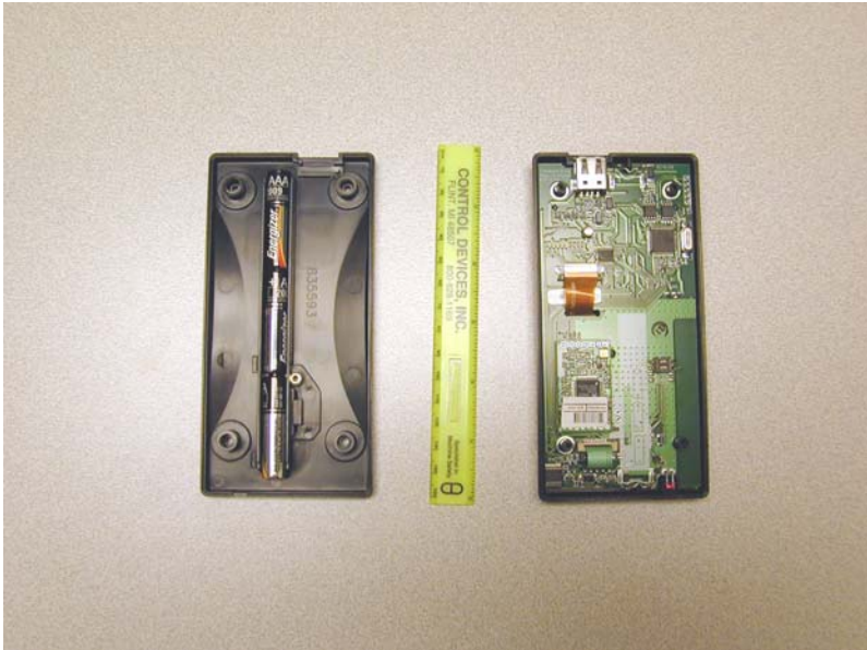
Keypad Case Inside
