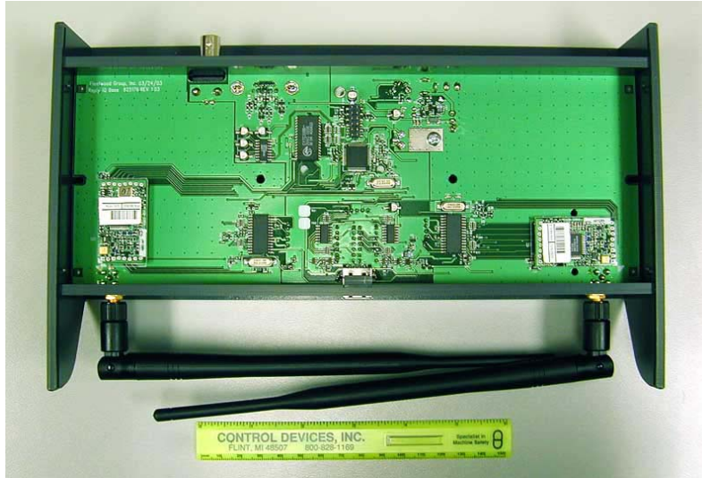
Base Circuit Board Component Side
