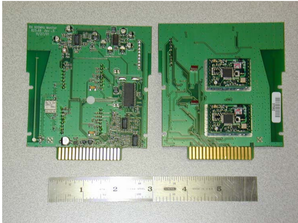
ECM9XX Monitor Receiver circuit board top and bottom views
