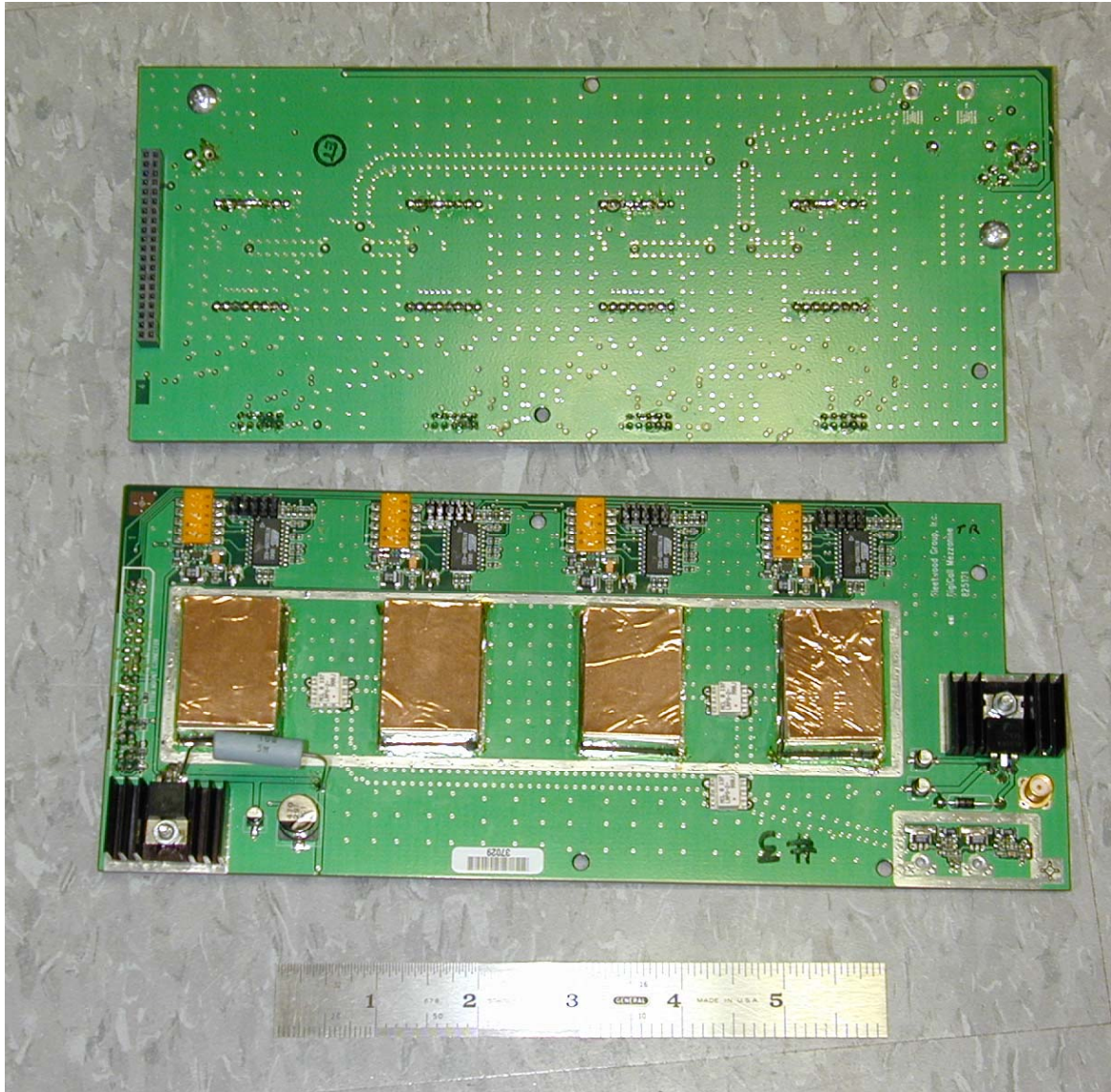
ECM9XX Mezzanine circuit board top and bottom views
