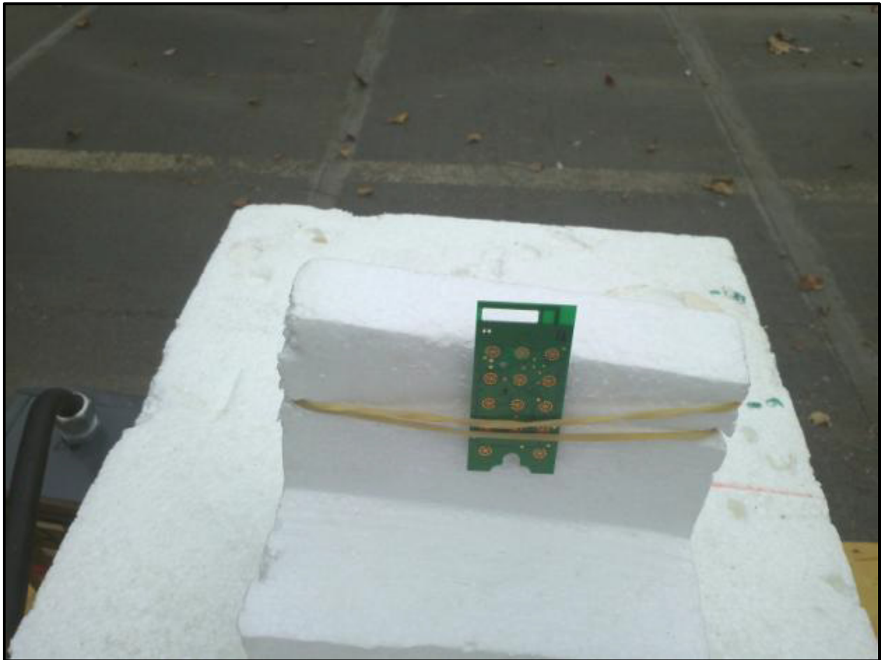
Photograph 6: Radiated Testing – Front View – Standalone – Standard XTAL
