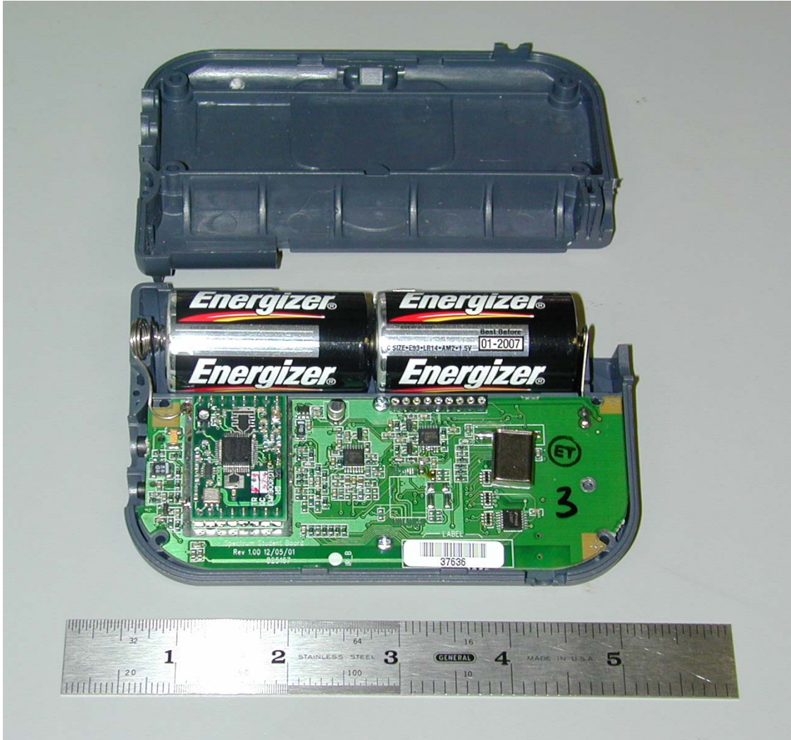
DS6MA Student Transceiver Case Internal Top and Bottom Views
