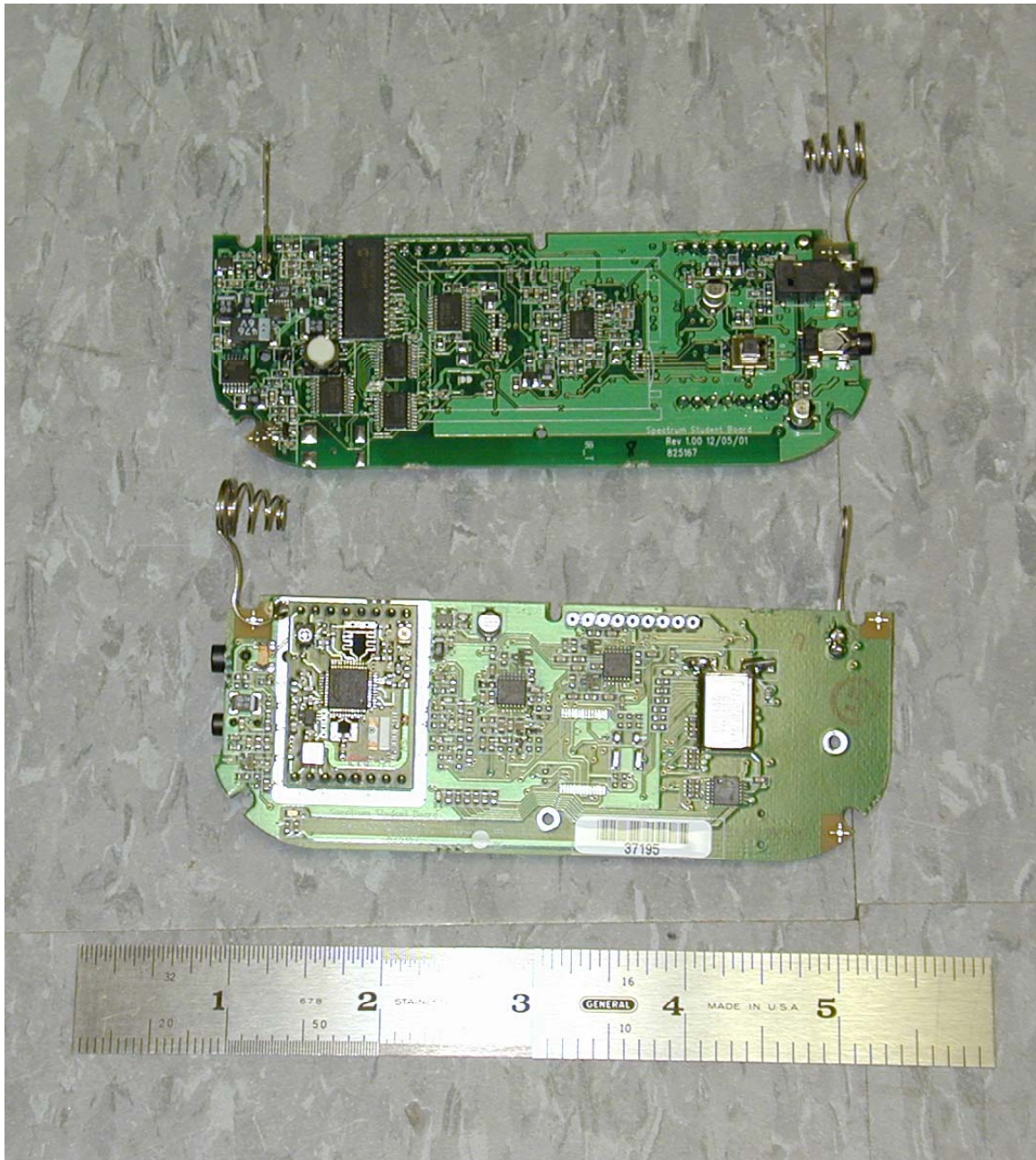
DS6MA Student Transceiver Circuit Board Top and Bottom Views
