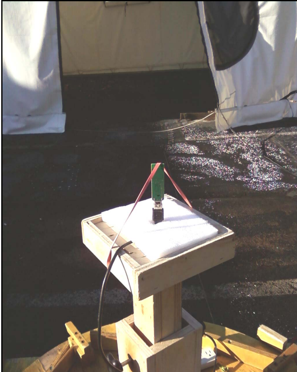
Photograph 4: Radiated Testing – Back View
