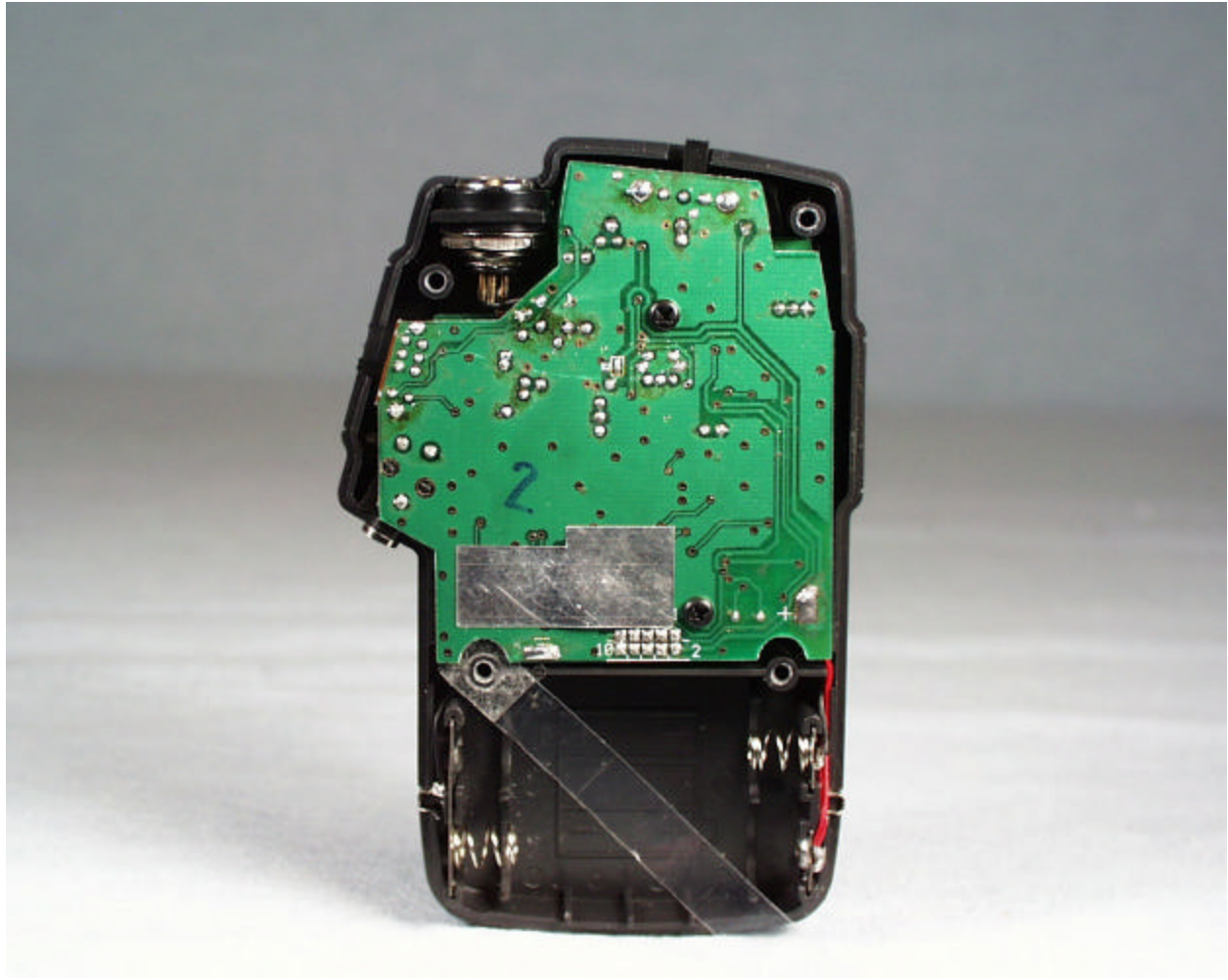
Side A of the Venture-Express (Main board)
