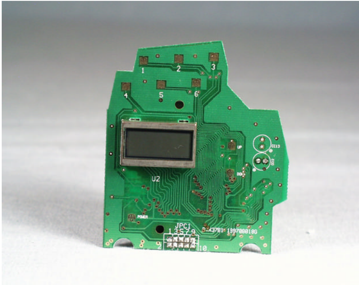
Side B of the Venture-Express (CPU board)
