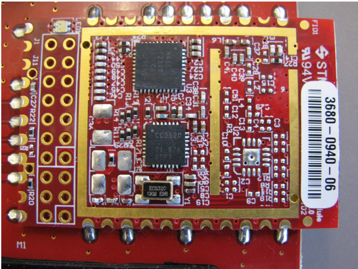
Photograph 5 - Component Side of the RF Daughter Card
