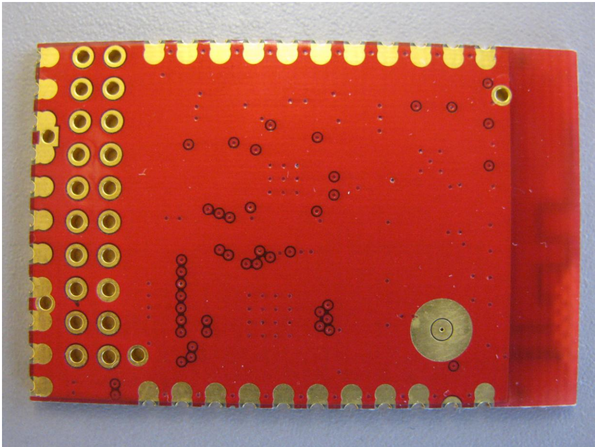
Photograph 6 - Trace Side of the RF Daughter Card
