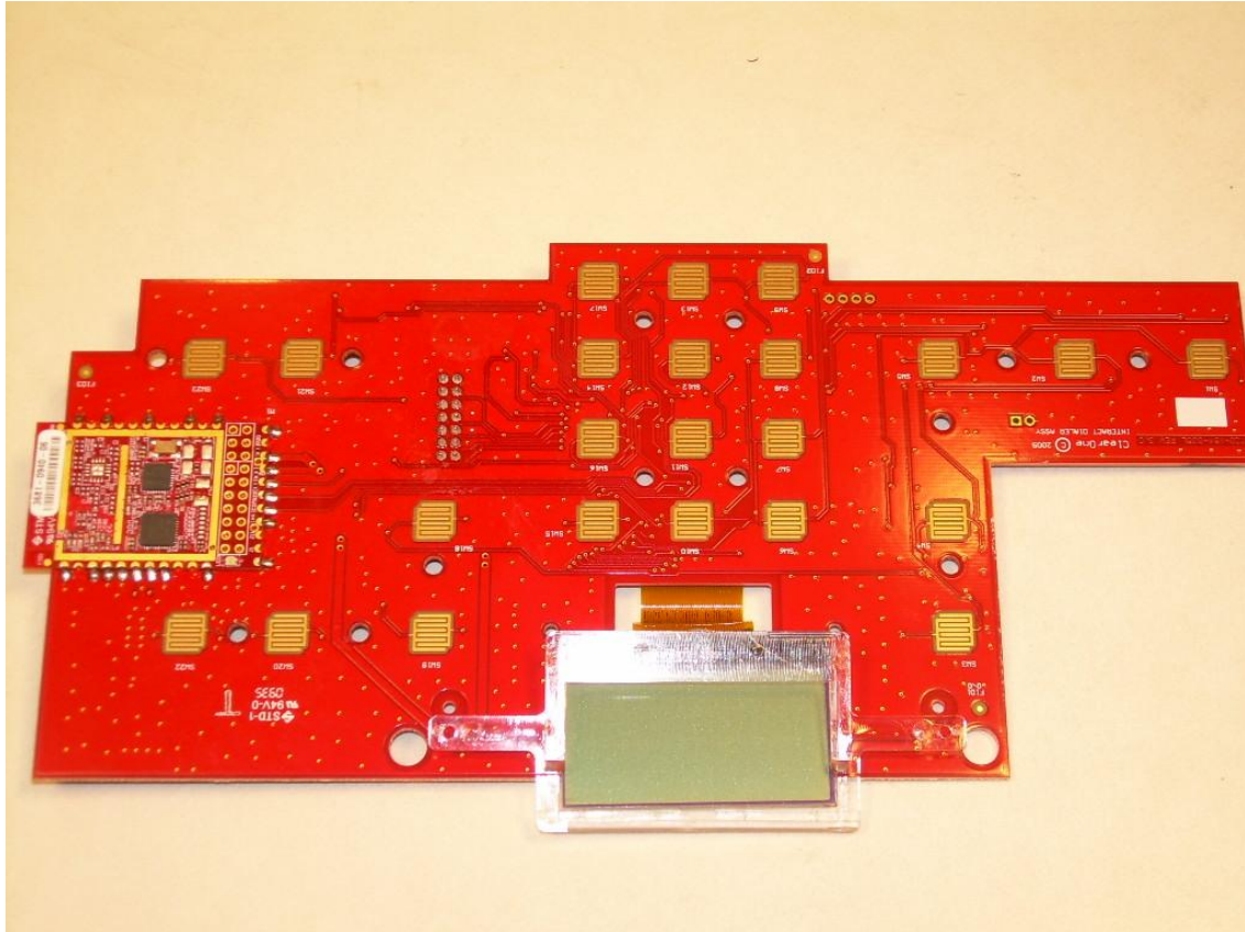
View of the Top of the PCB
