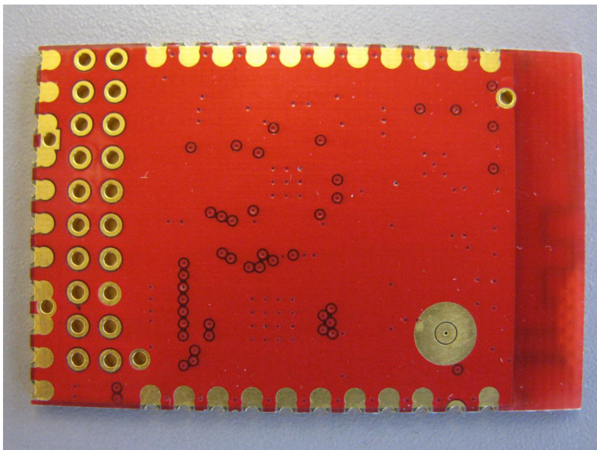
Trace Side of the RF Daughter Card
