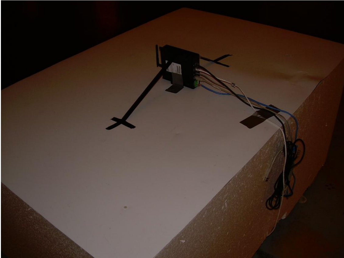
View of the Radiated Spurious Emission Configuration - On-Edge
