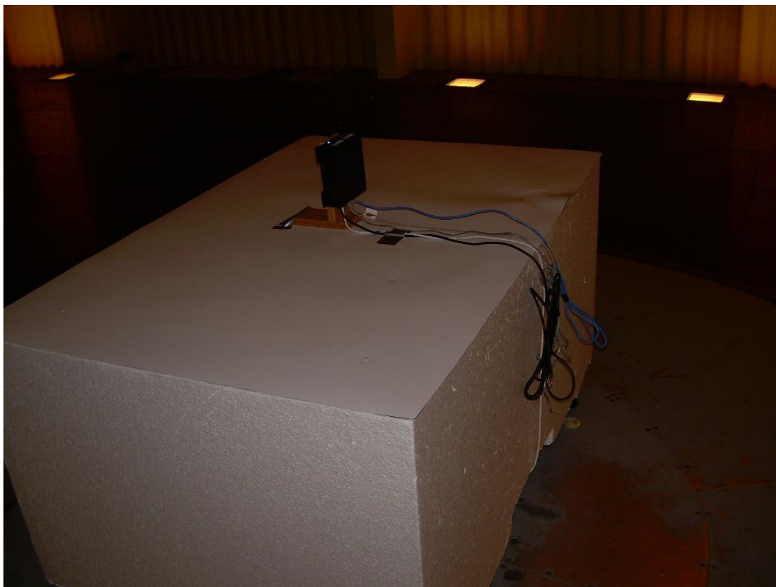
View of the Radiated Spurious Emission Configuration - Vertical
