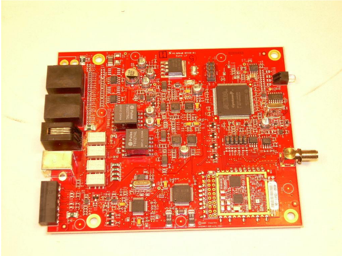
Component Side of the COM-W PCB
