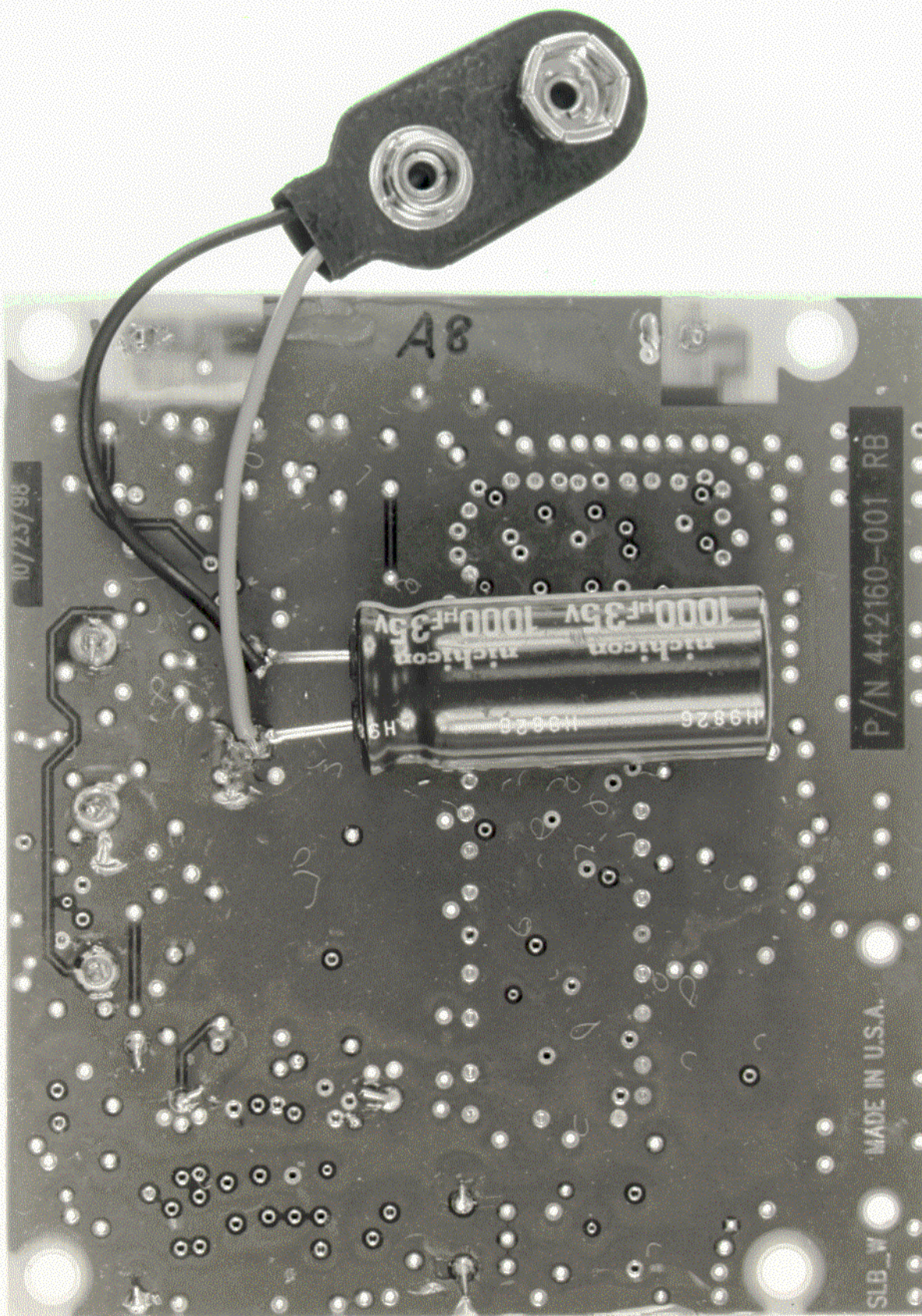
Schlumberger FCC ID: F9CTALWCNMIU1 Transmitter PCB Bottom
