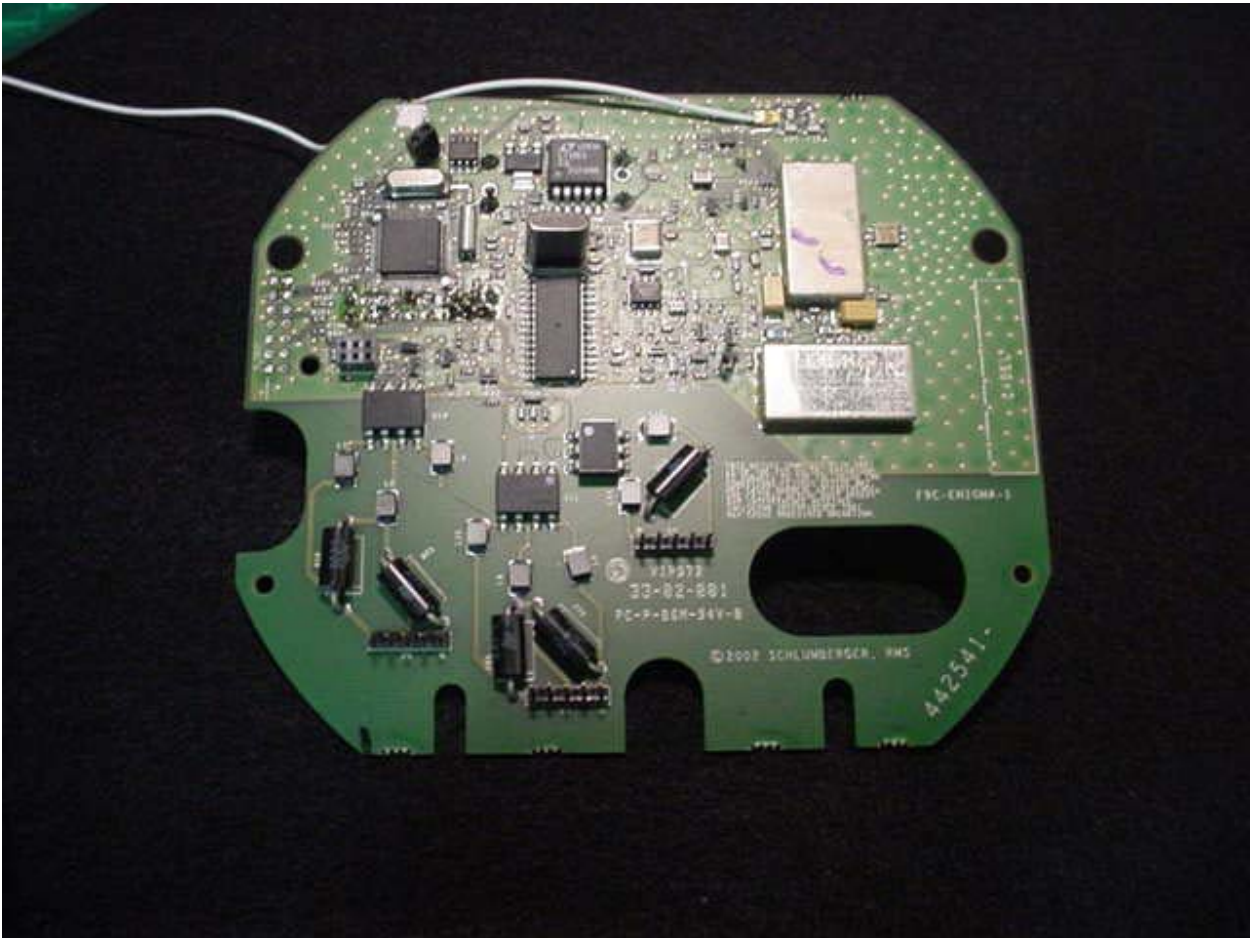
Figure B5: Top Side of RF Board
