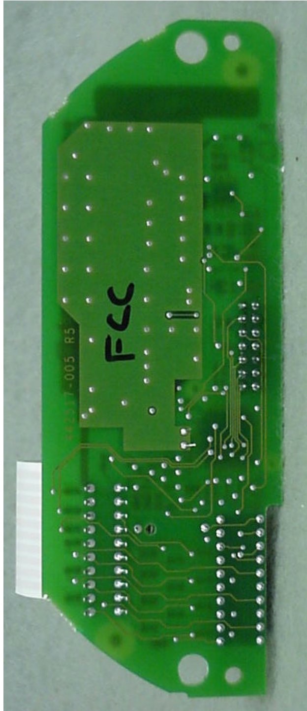
Photo 12. EUT, Bottom View of Transmitter Board
