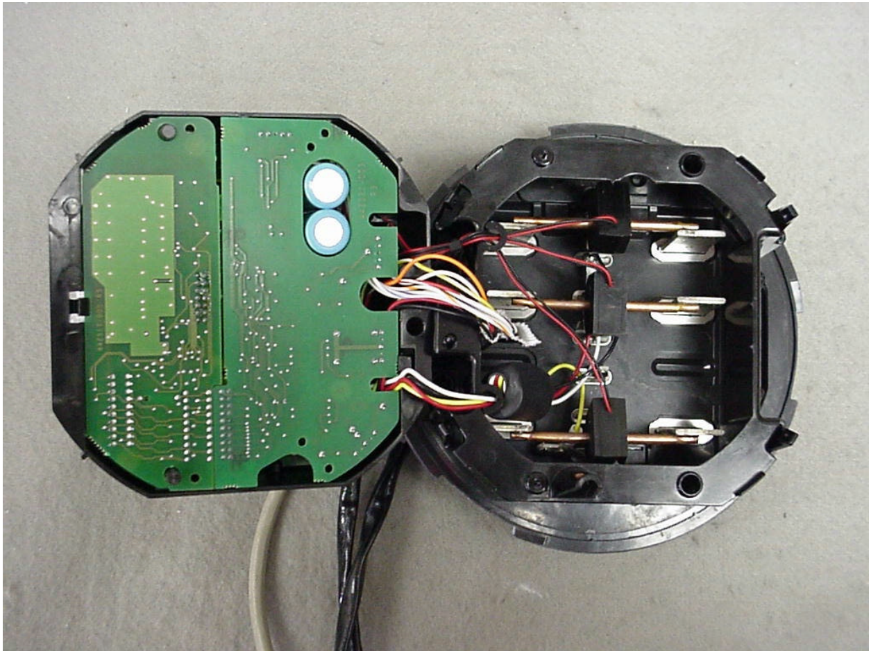
Photo 4. EUT, View with Electronics Removed
