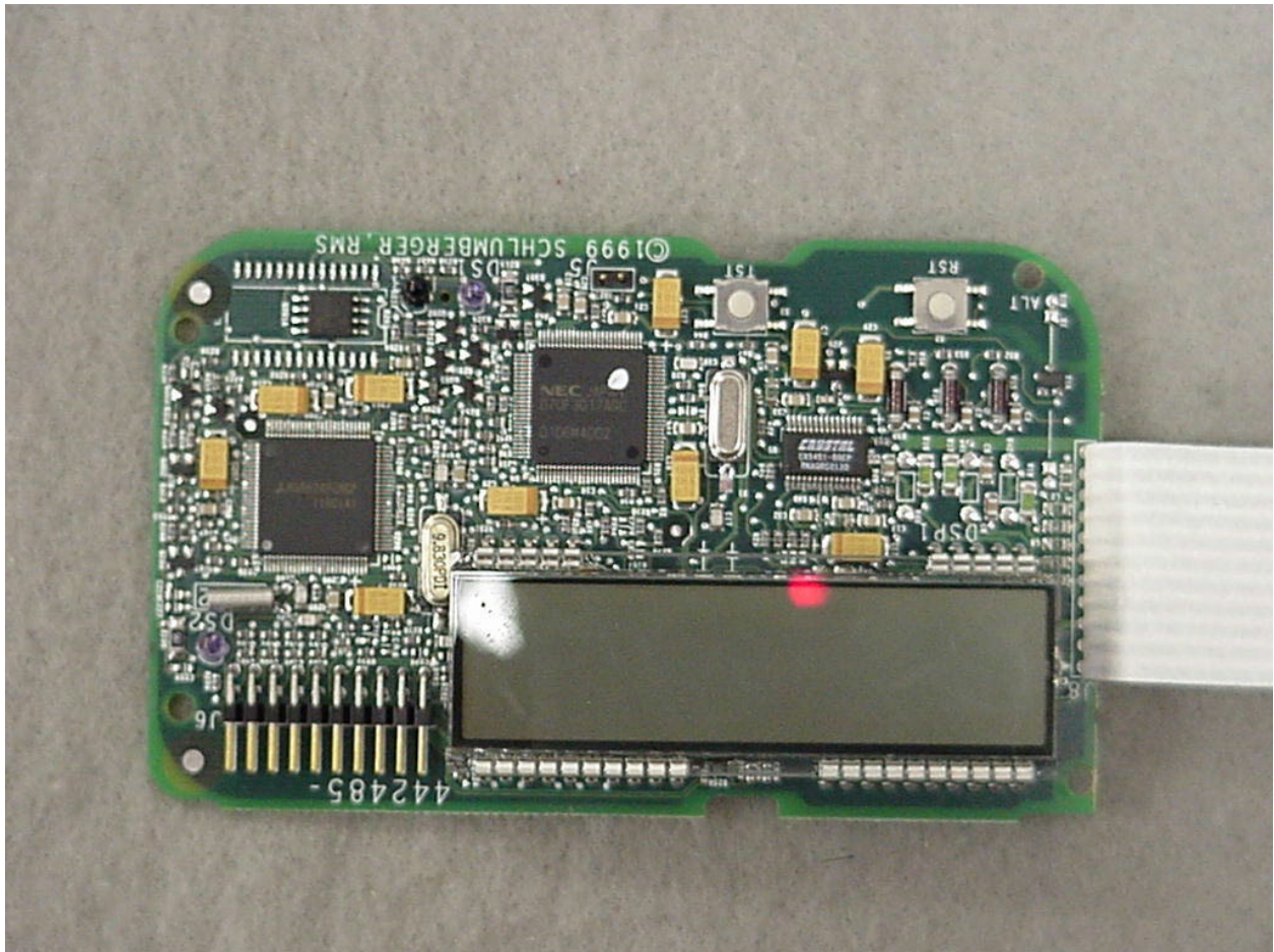
Photo 7. EUT, Top View of Register Board with LCD Display
