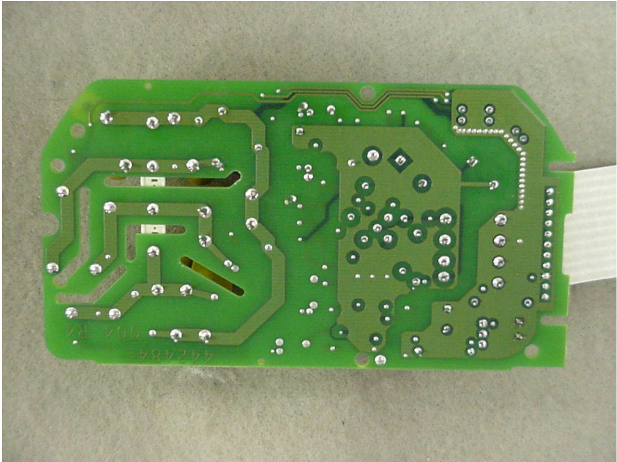
Photo 10. EUT, Bottom View of Power Supply Board
