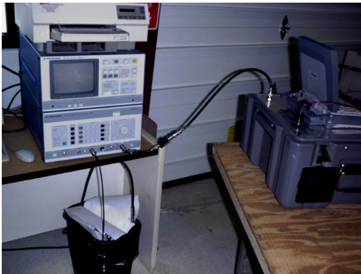
Photo : Conducted Measurements – View II
