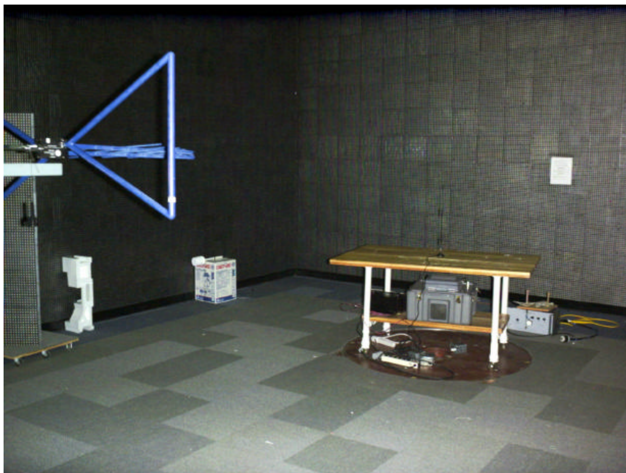
Photo : Radiated Measurements – View I
