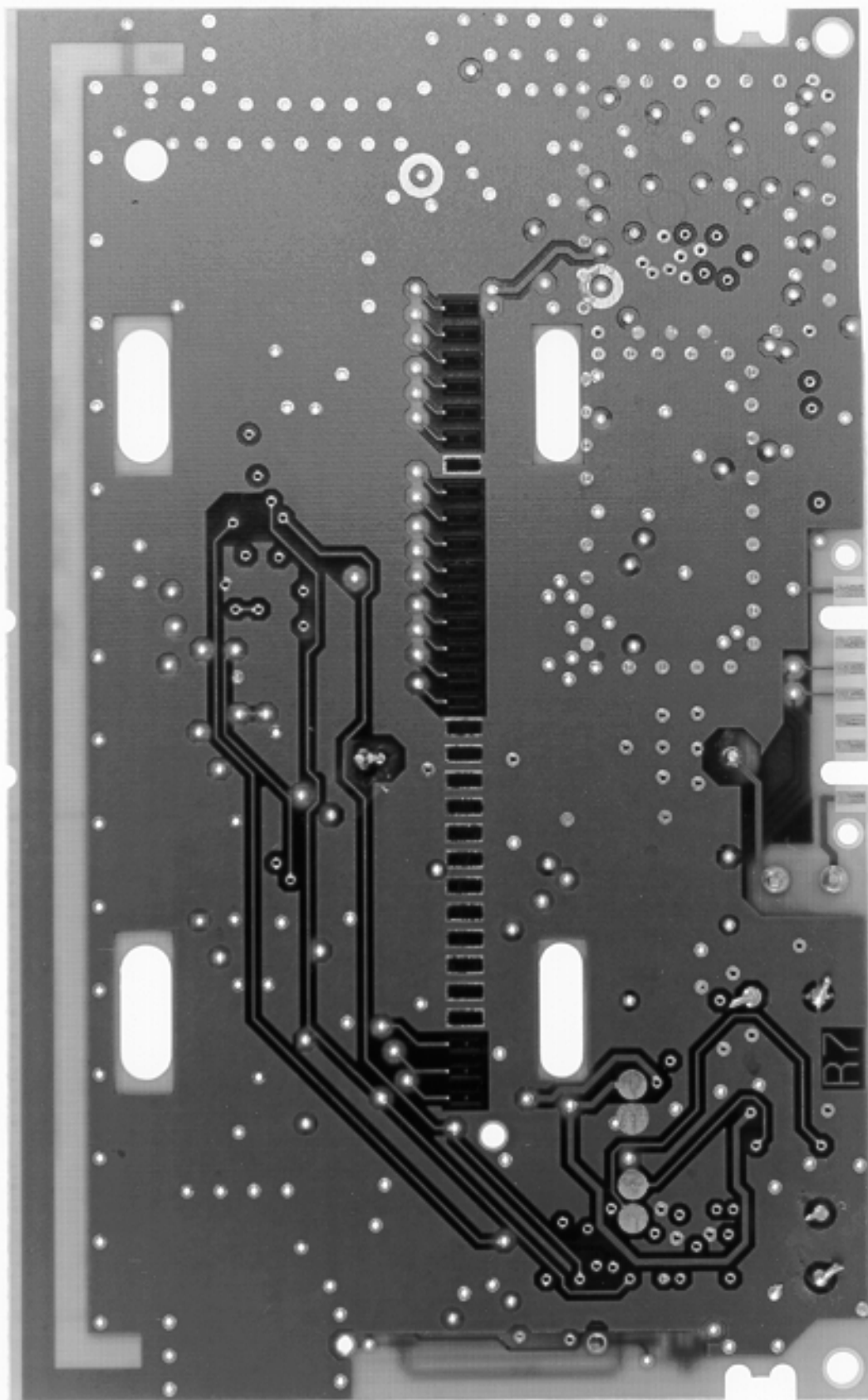
Schlumberger FCC ID: F9CC1C-1 Transmitter PCB Bottom View
