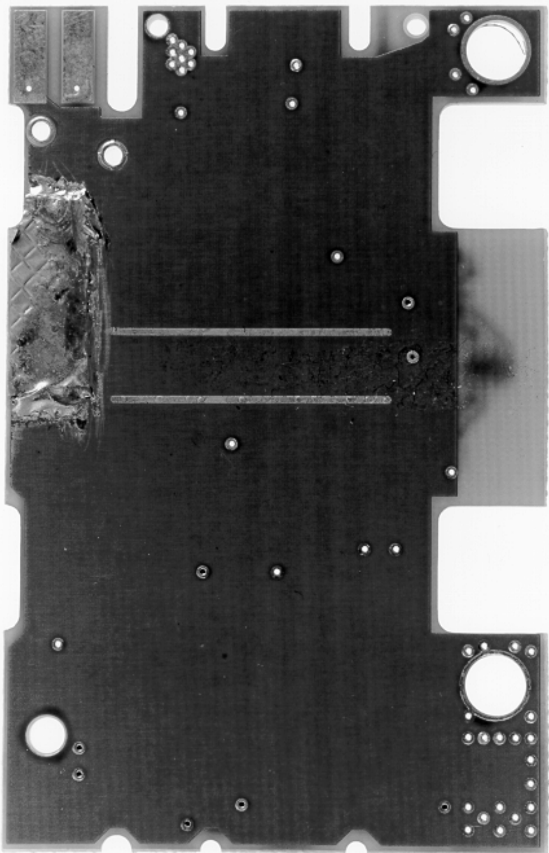
Schlumberger FCC ID: F9CC1C-1 Bottom PCB Bottom View
