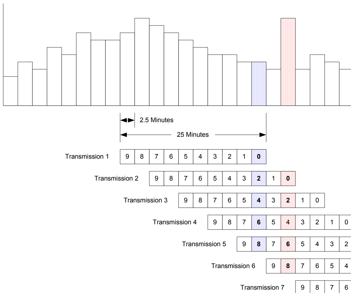
Figure 21 Cumulative 3 with 10 Intervals
