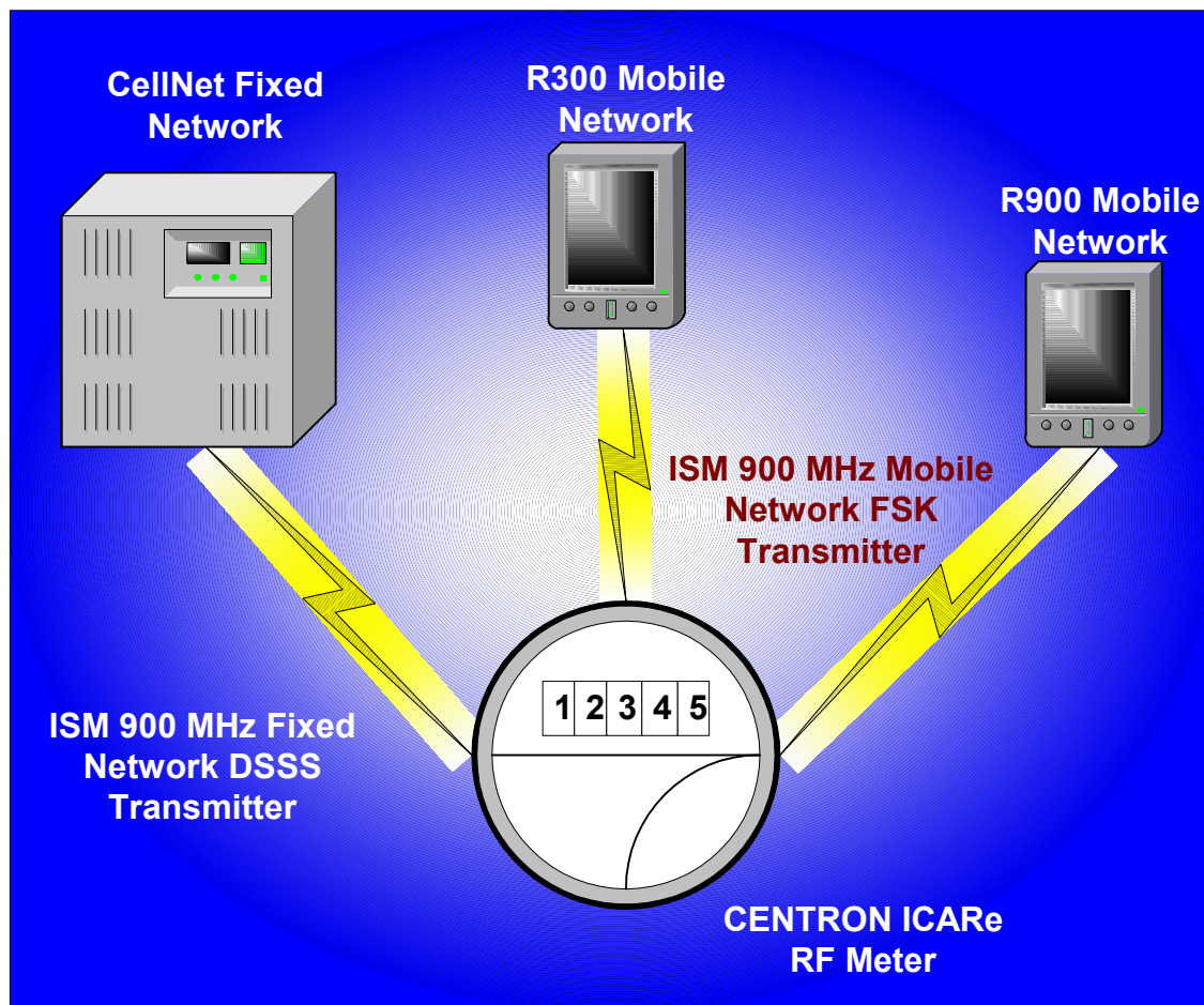
Figure 1 RF Network Interfaces
