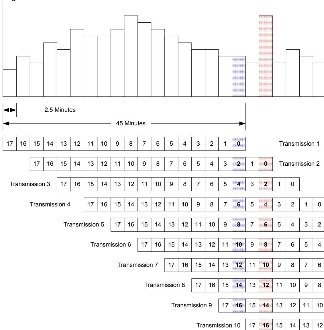
Figure 20 Cumulative 2 with 18 Intervals
