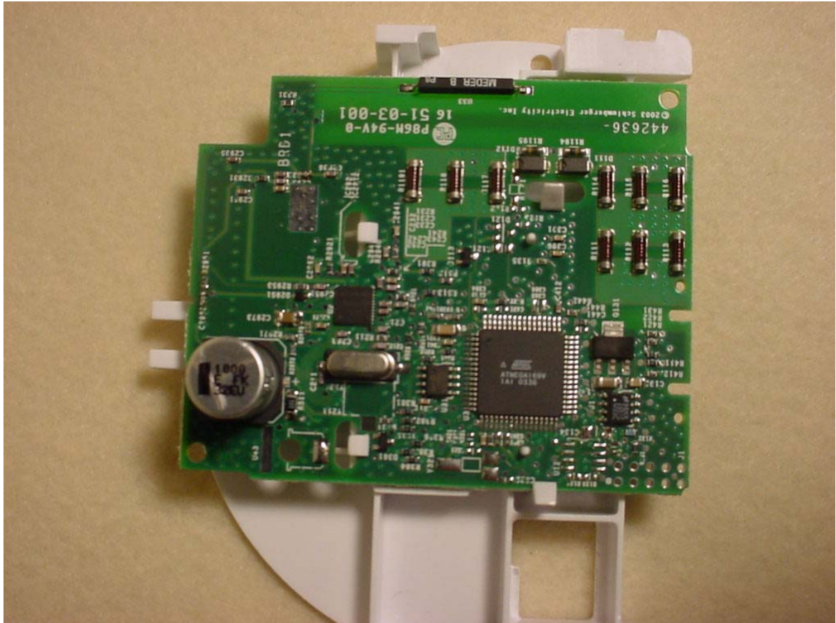
Figure 2: Circuit Board 1 – Top View
