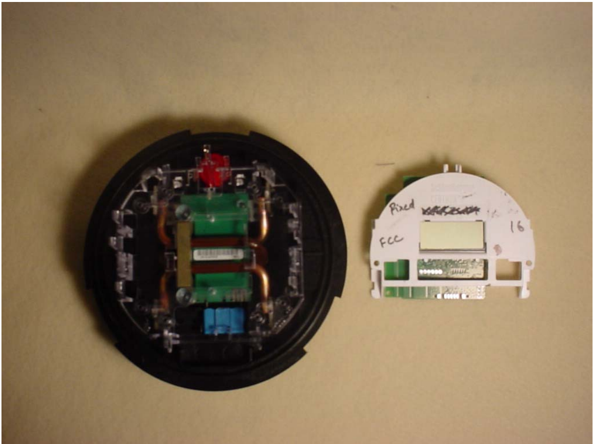
Figure 1: Internal – Front View
