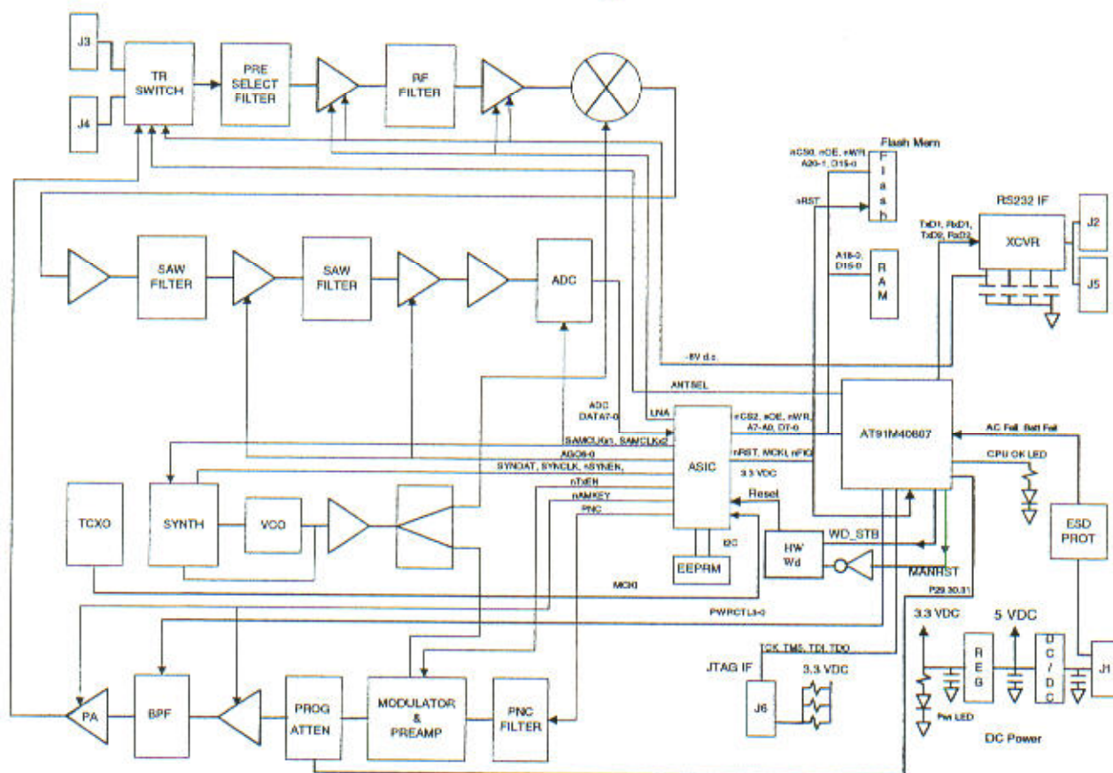
Figure 1, BLT III Hardware Block Diagram
