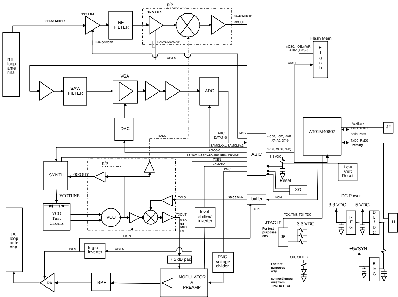
eT HARDWARE BLOCK DIAGRAM, 23 JANUARY 2001
