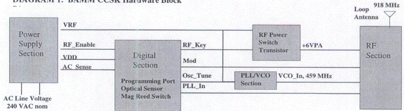
DIAGRAM 1: BAMB CCSK Hardware Block
