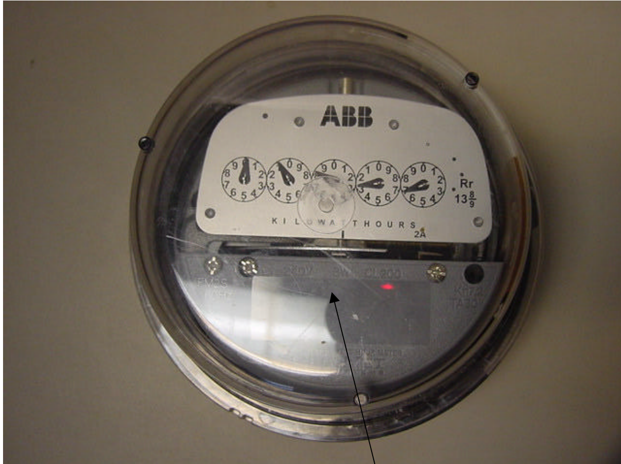
Location of transmitter board installed underneath the plastic enclosure FRONT SIDE OF METER (1 OF 2)
