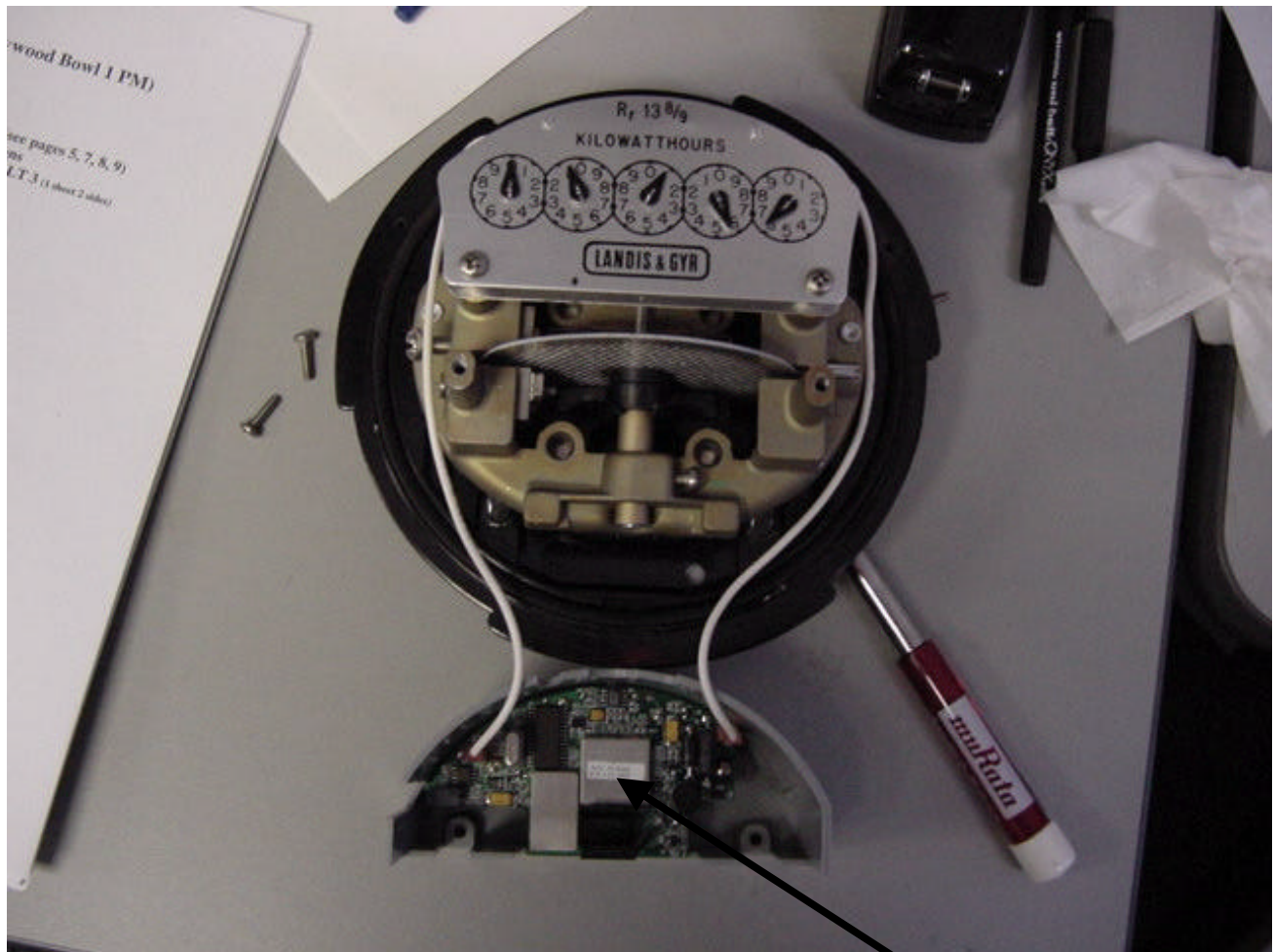
Plastic enclosure with Transmitter board exposed FRONT SIDE OF METER (2 OF 3)
