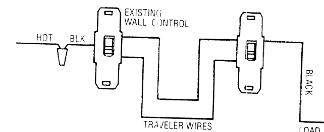
3-WAY WIRING DIAGRAM: RETROFIT
