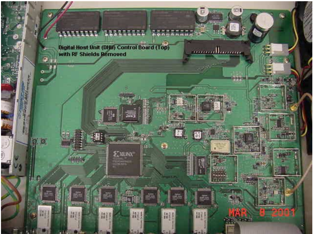
DHU BOARD TOP NO SHIELDS
