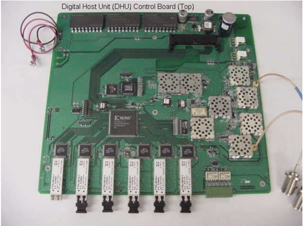
DHU board top
