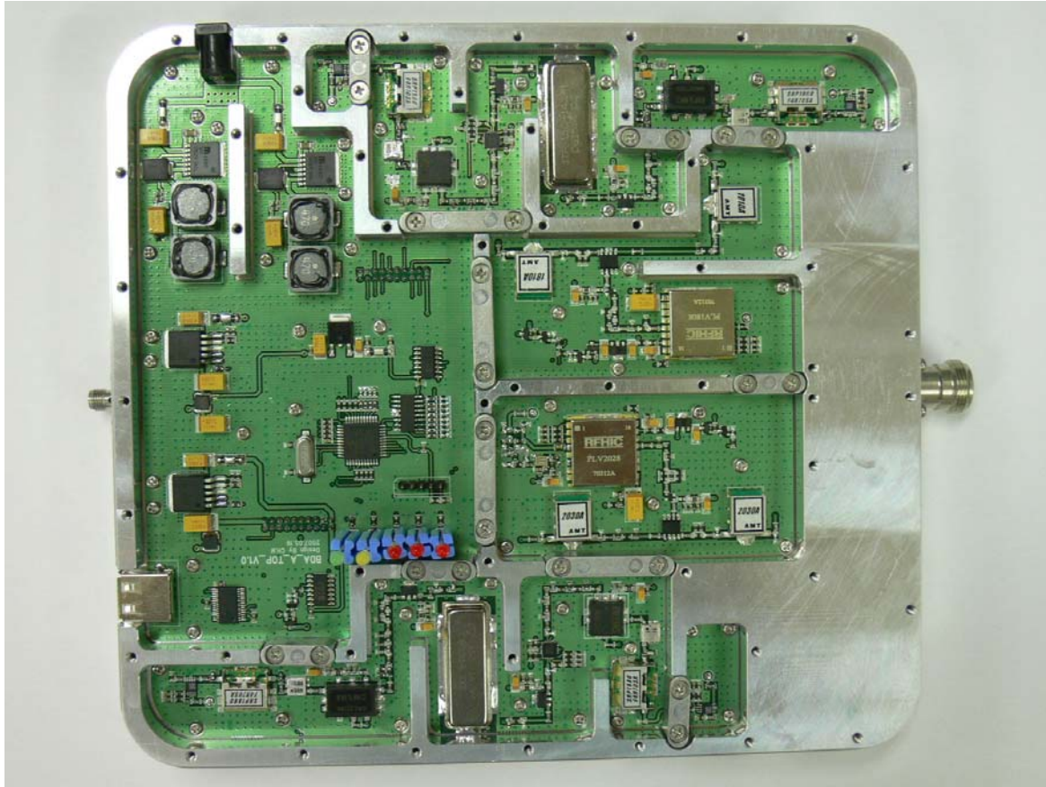
INTERNAL PHOTOS PCB 1 - Installed
