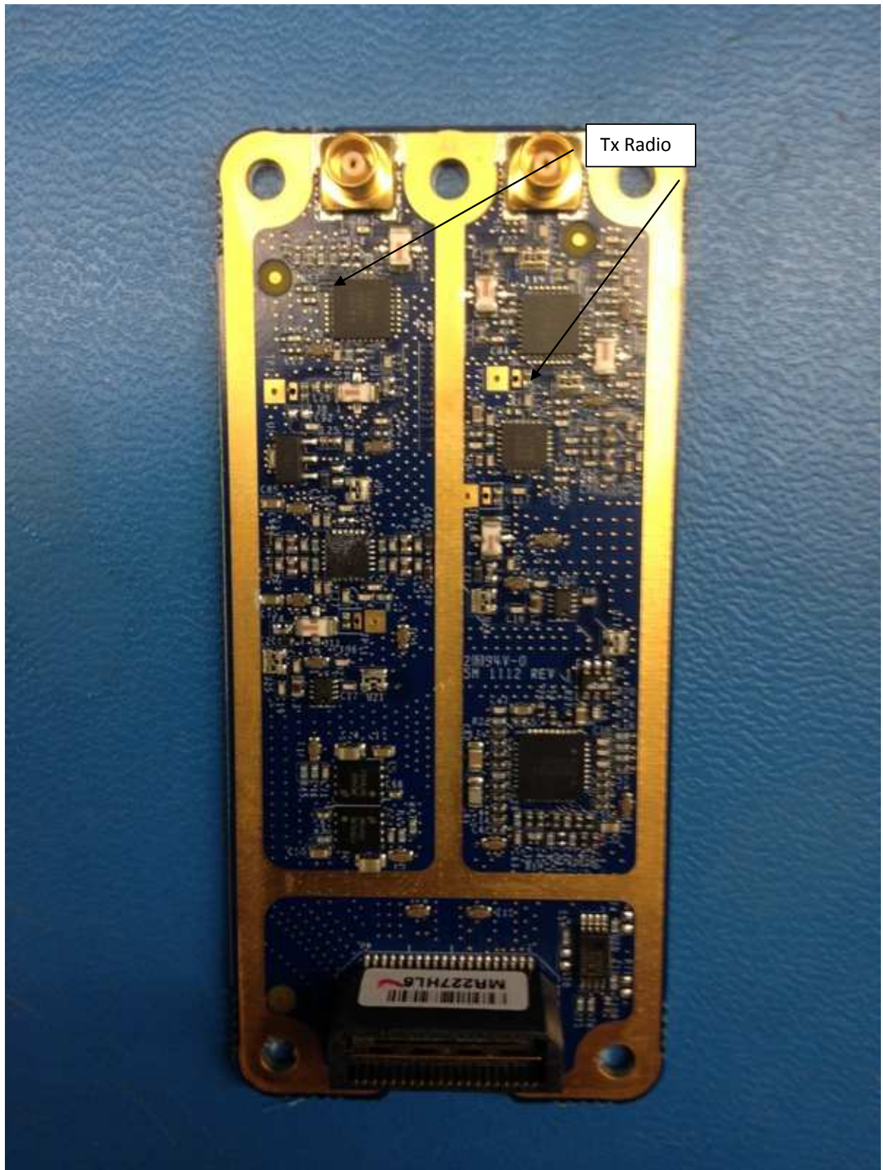
Tx Board – Front
