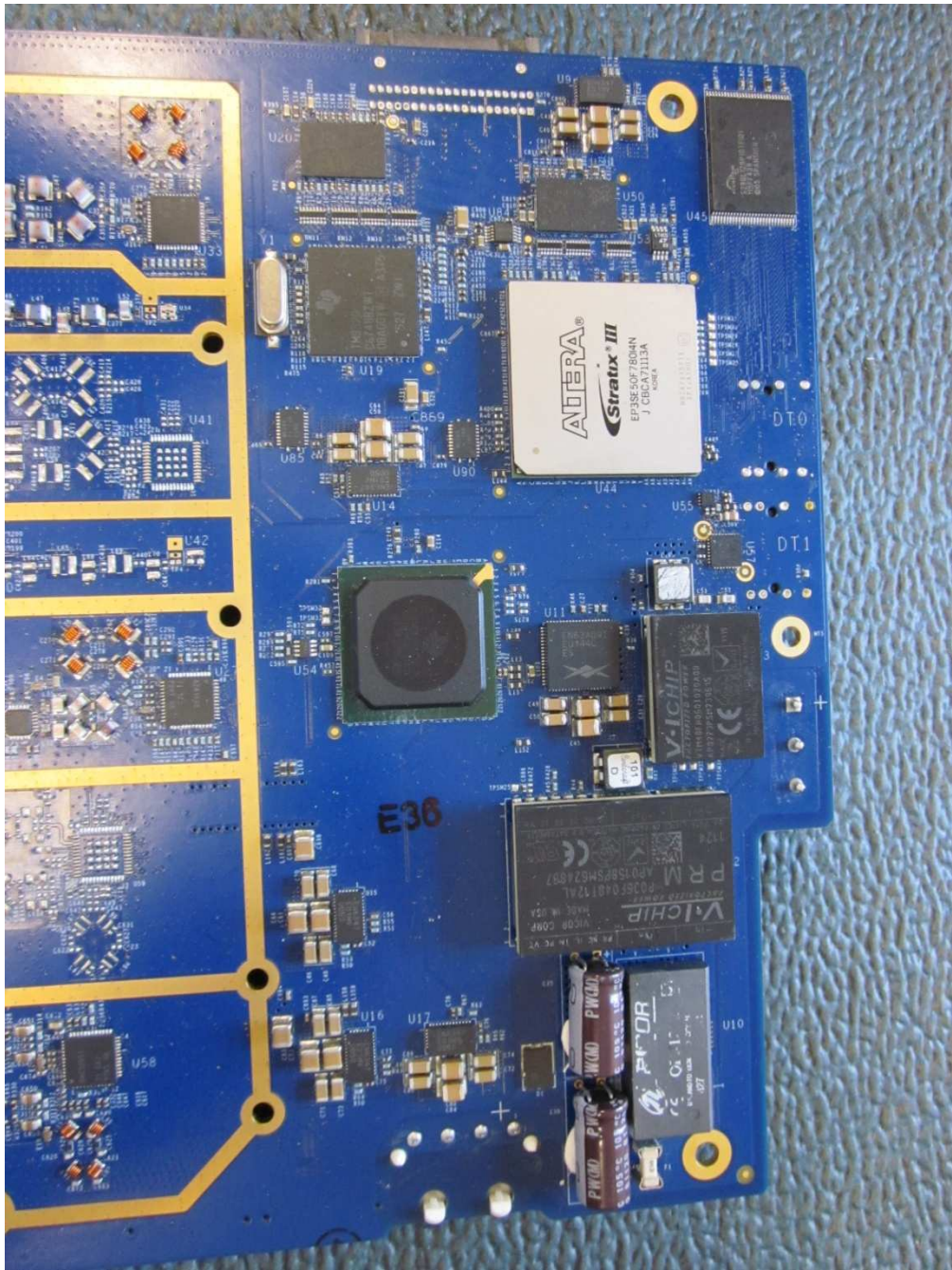
Motherboard – Front #3
