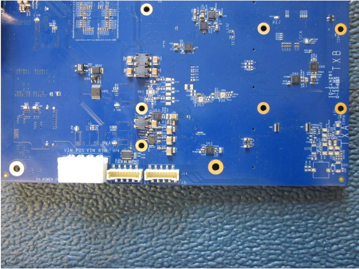
Motherboard – Back #2
