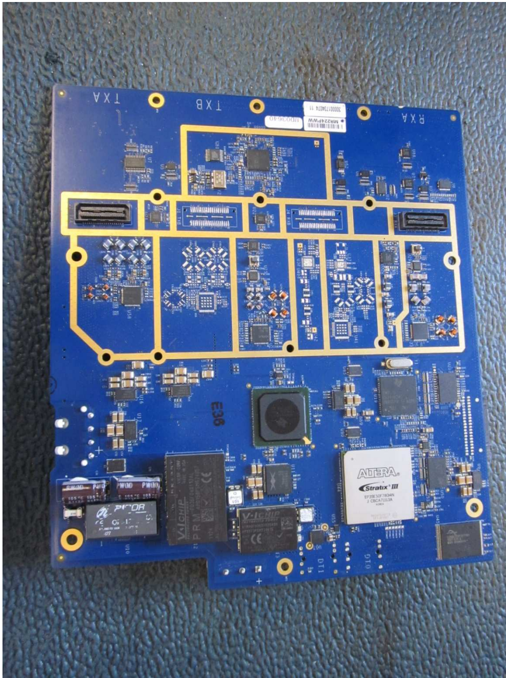
Motherboard – Front #1
