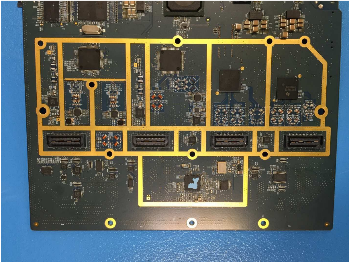
Motherboard – Back #2
