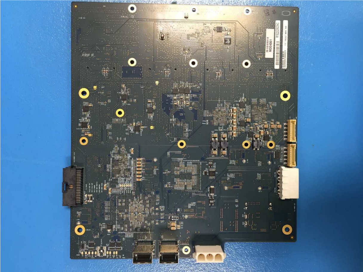
Motherboard - Front
