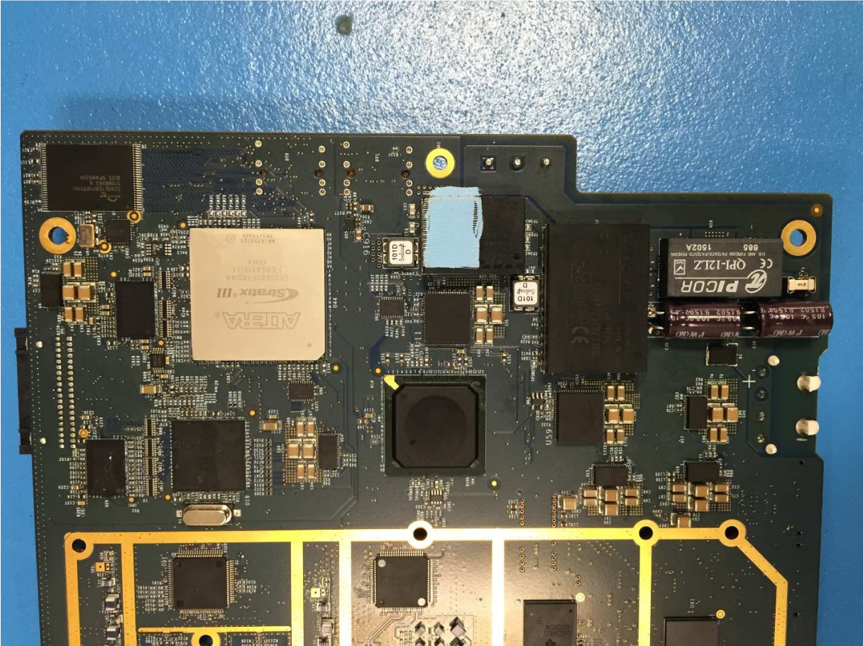
Motherboard – Back #3
