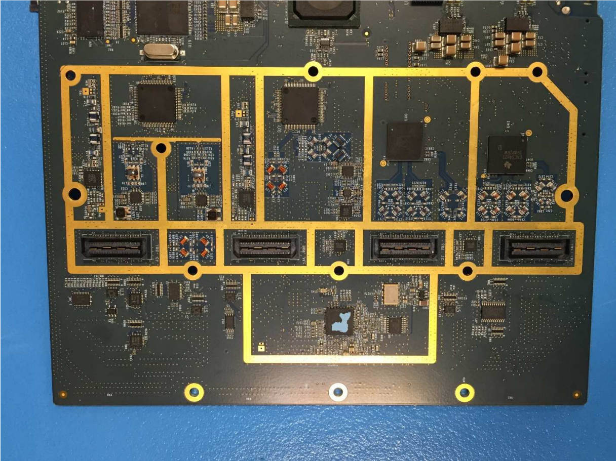
Motherboard – Back #2
