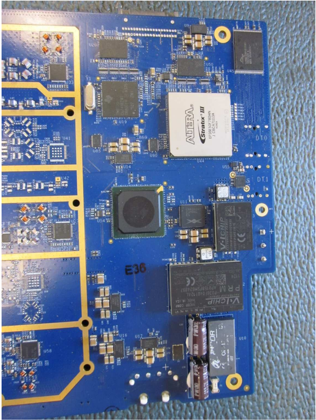
Motherboard – Front #3
