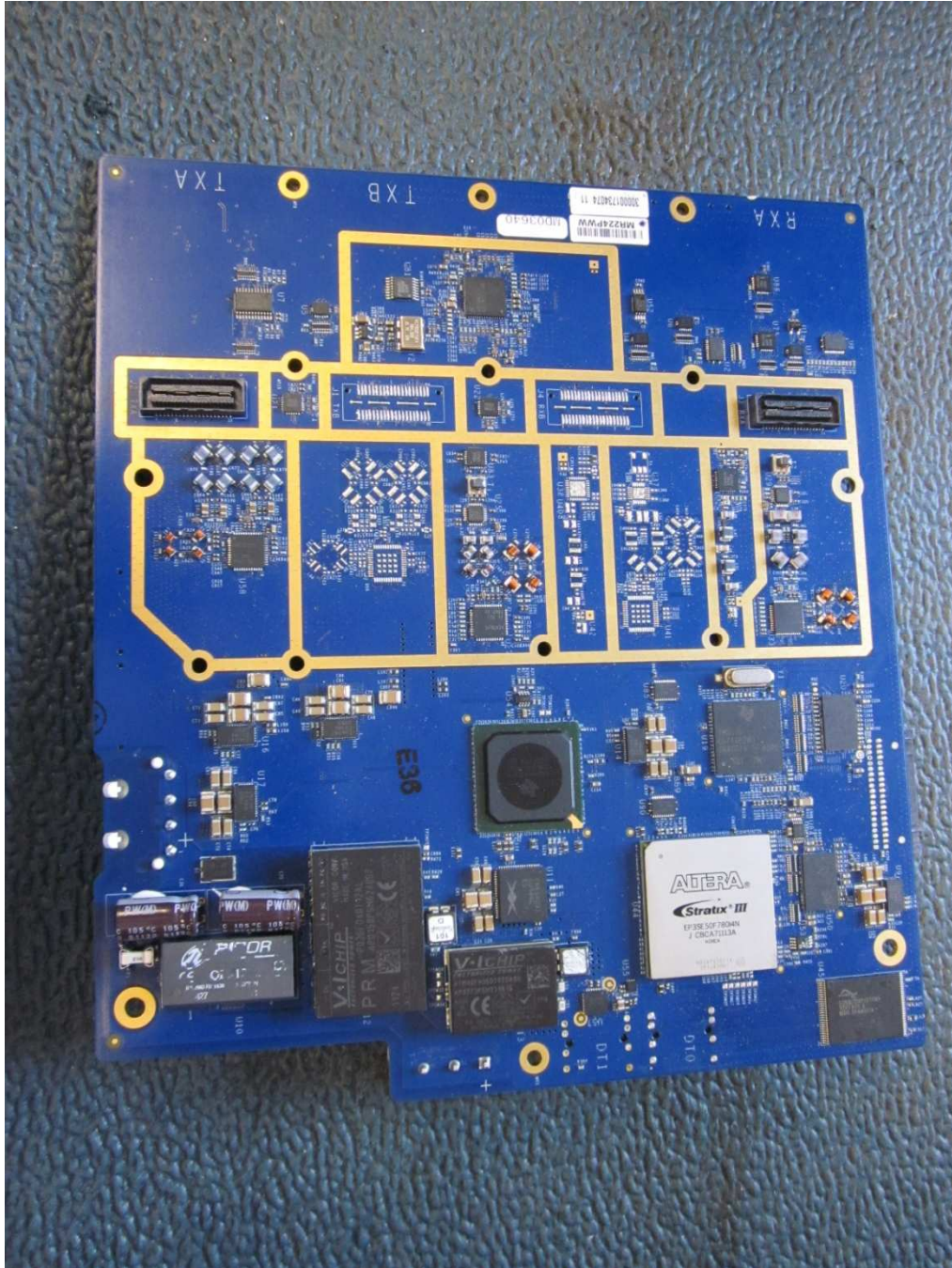
Motherboard – Front #1
