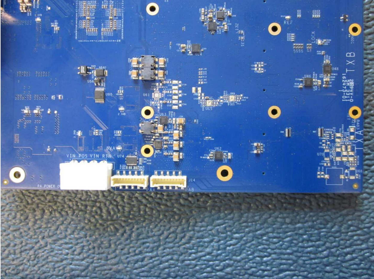
Motherboard – Back #2
