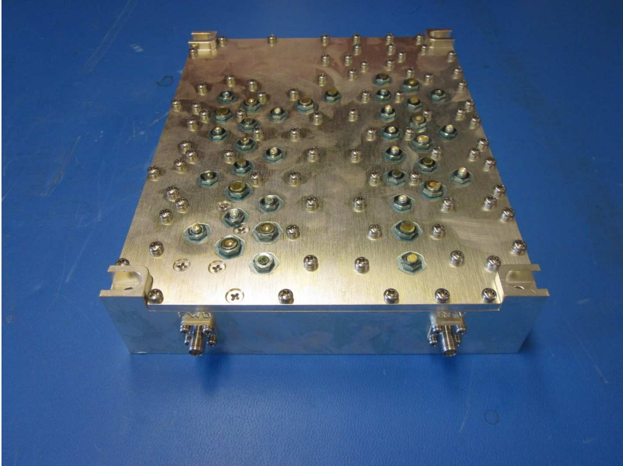
Duplexer #1
