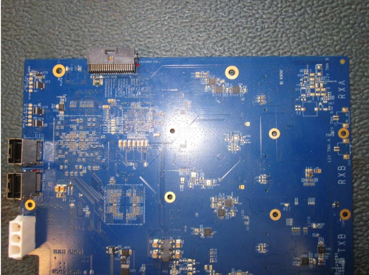
Motherboard – Back #3
