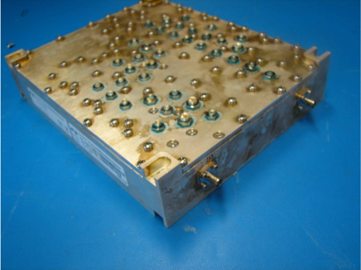
Duplexer #3
