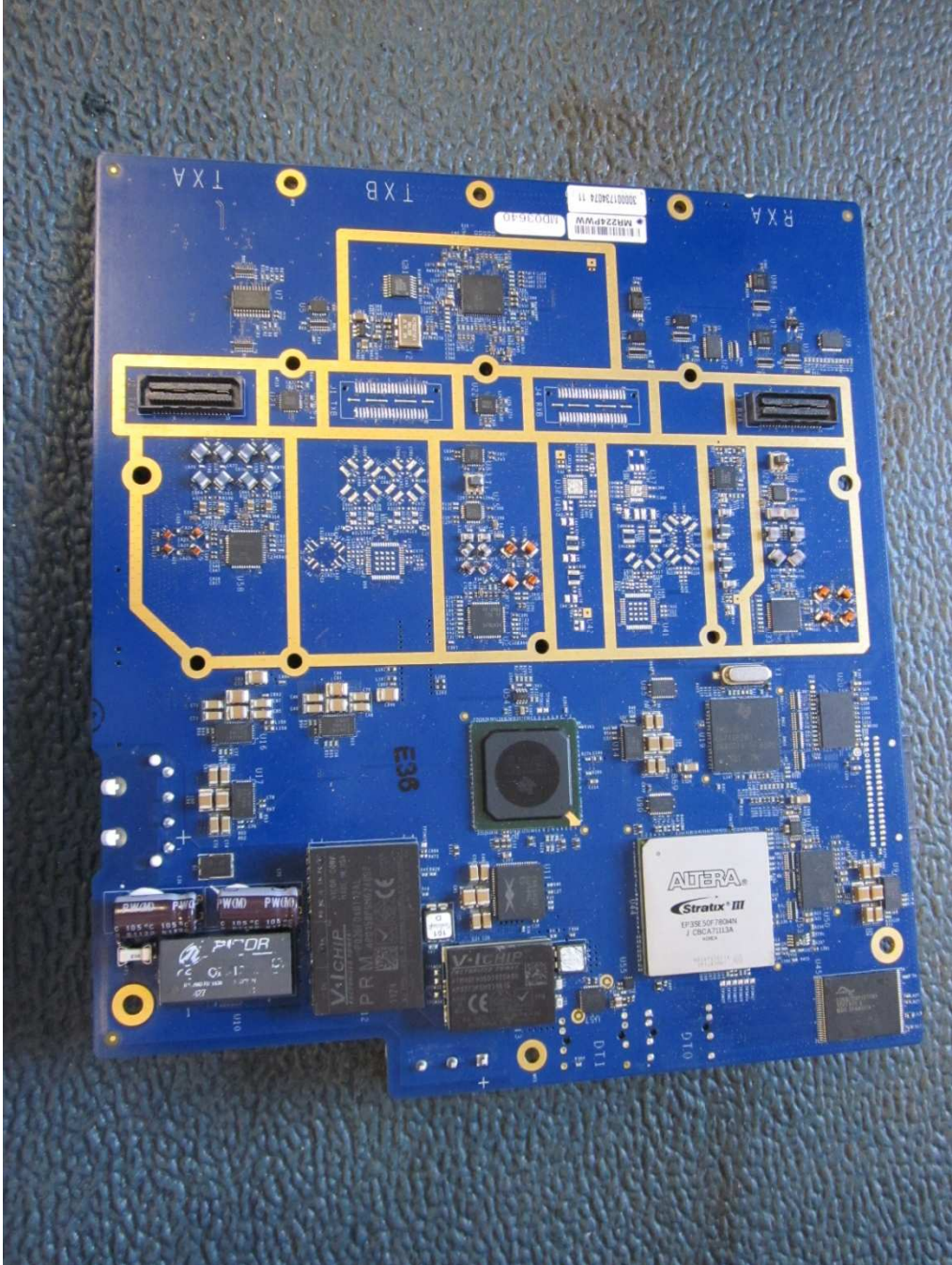
Motherboard – Front #1
