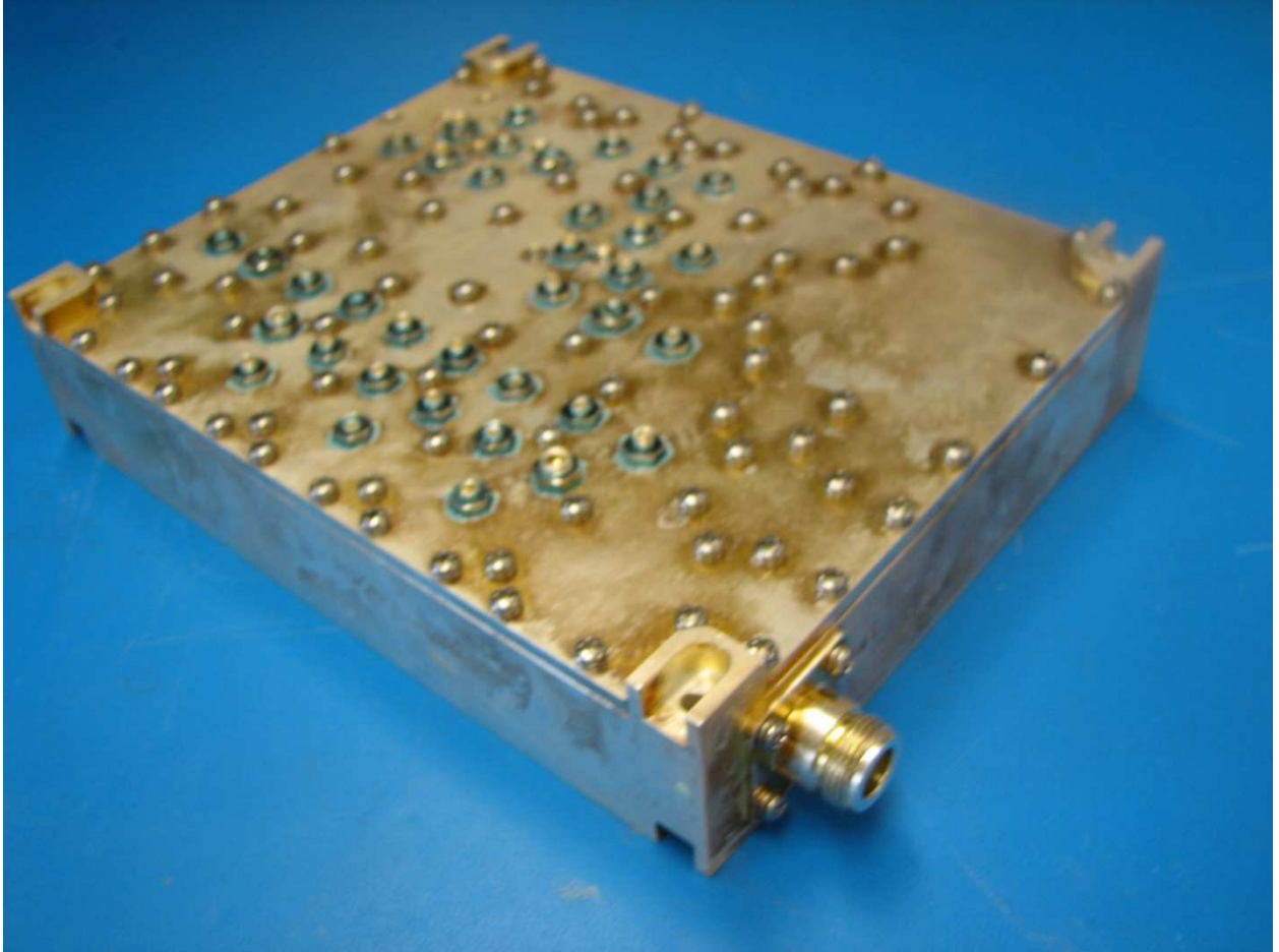
Duplexer #2
