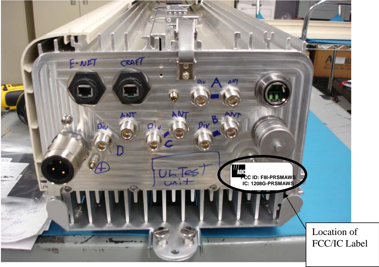
FlexWave™ Prism - AWS Remote Unit Location of FCC/IC ID
