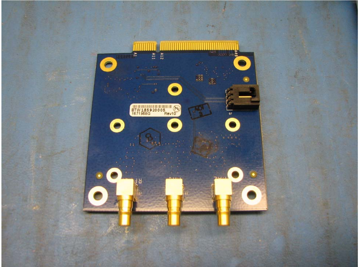
40 Watt Prism Vector Modulator Board (top)
