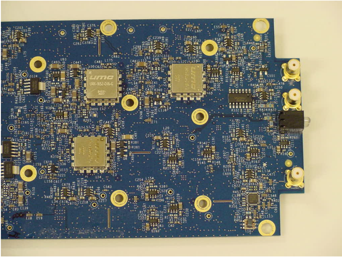
FlexWave™ URH DART Top View - 2
