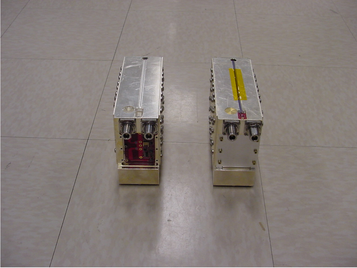
FlexWave™ URH Duplexer - PCS Rear View
