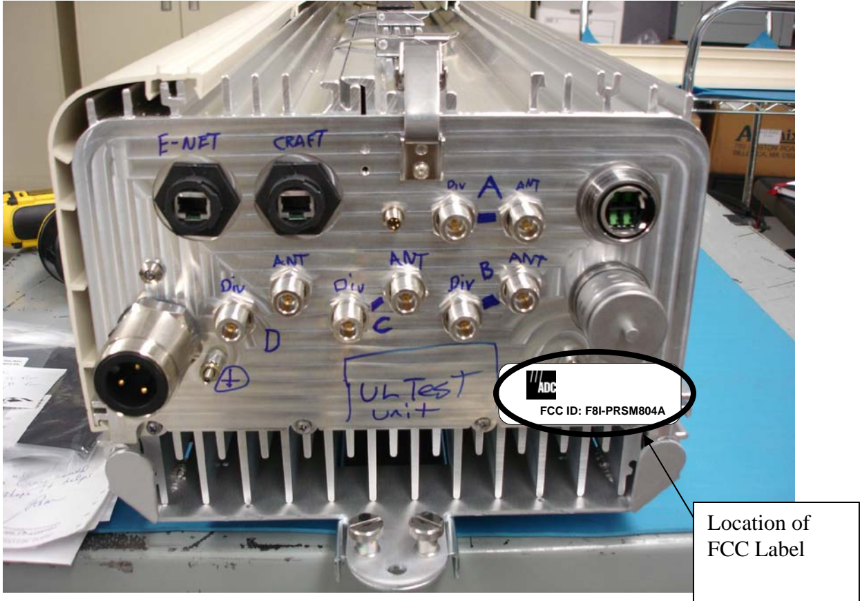
FlexWave™ Prism - Cellular 40W Remote Unit Location of FCC ID
