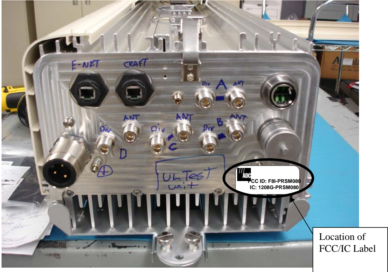
FlexWave™ Prism - Cellular Remote Unit Location of FCC/IC ID
