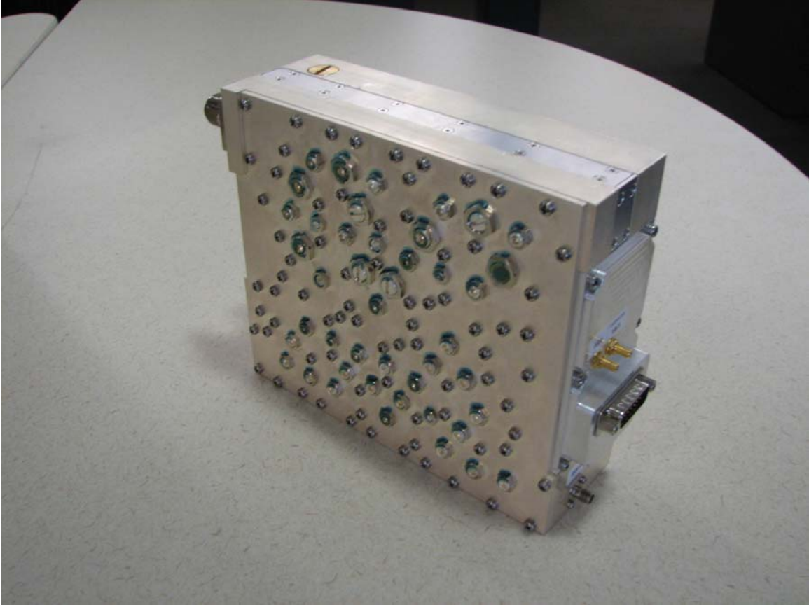
FlexWave™ Prism Duplexer - 700 Lower ABC Left View
