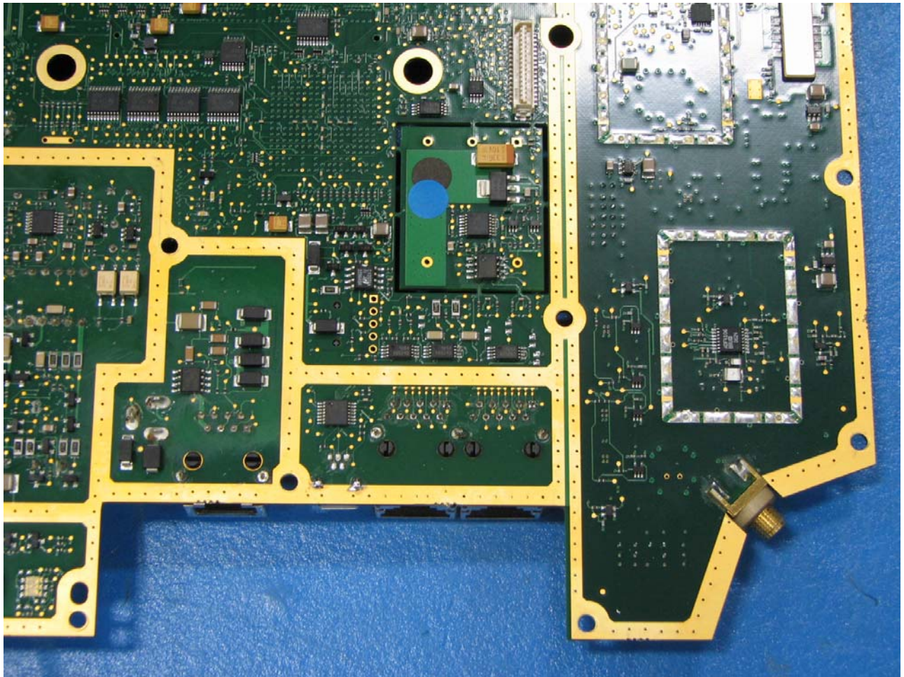
IP Access nanoBTS Bottom View – Lower Right
