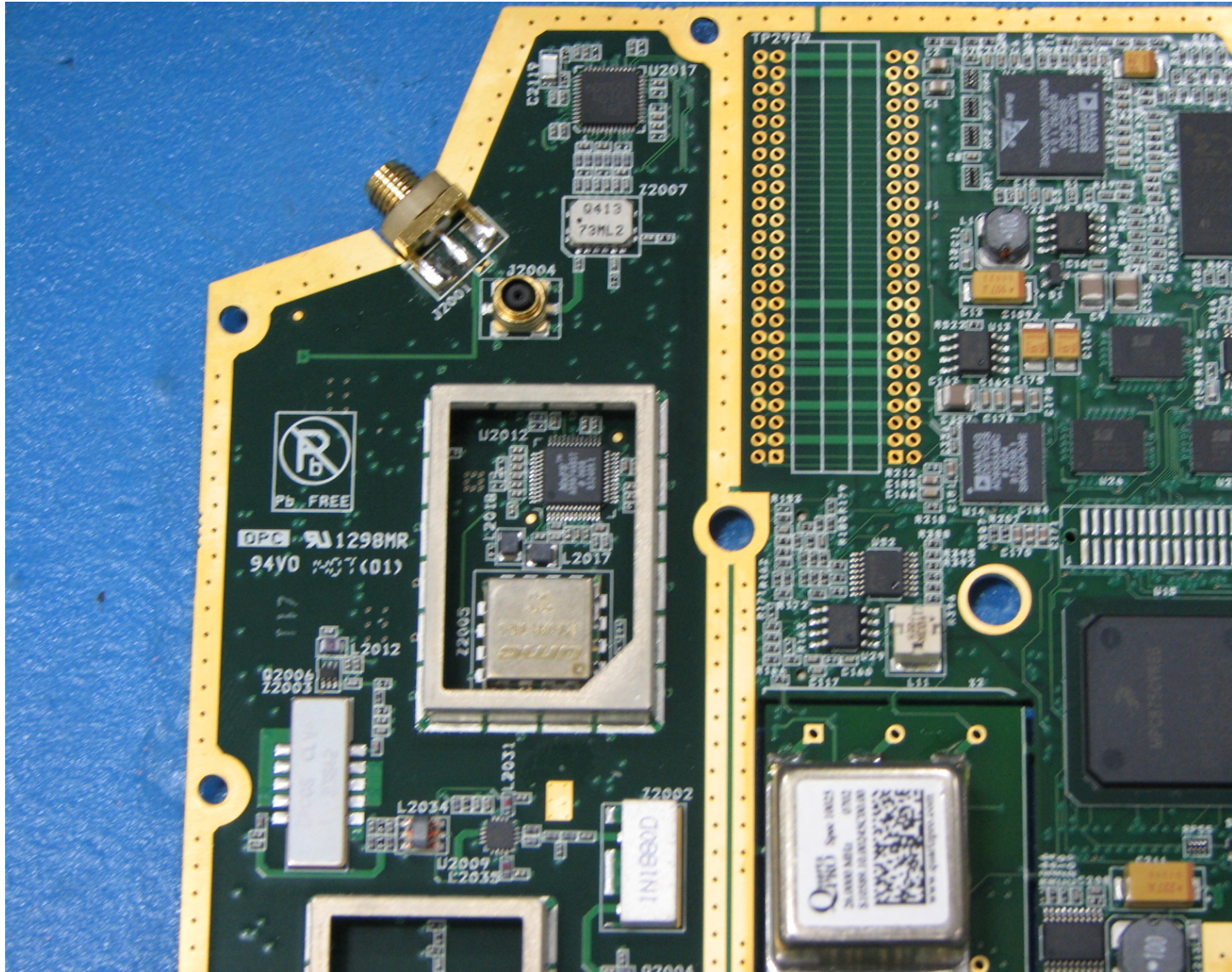
IP Access nanoBTS Top View – Upper Left
