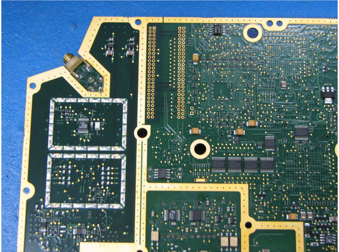
IP Access nanoBTS Bottom View – Upper Left
