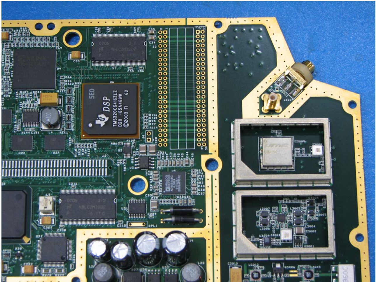
IP Access nanoBTS Top View – Upper Right
