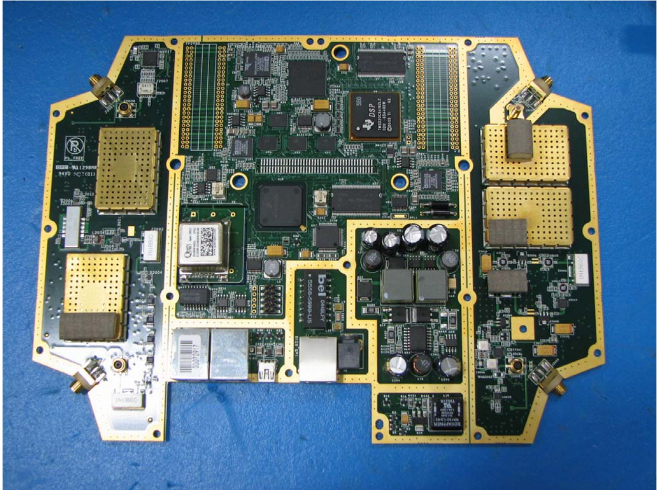
IP Access nanoBTS Top View
