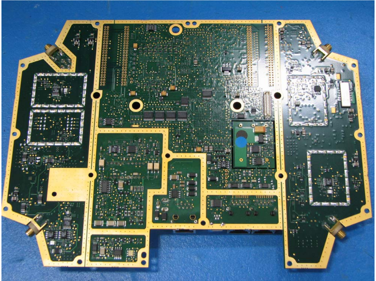
IP Access nanoBTS Bottom View
