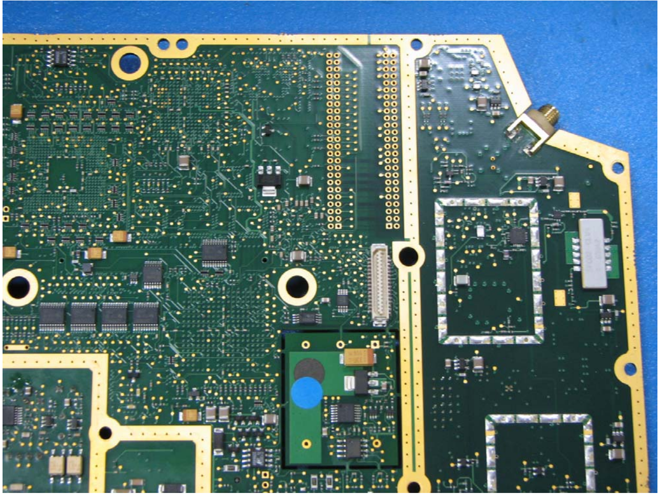
IP Access nanoBTS Bottom View – Upper Right
