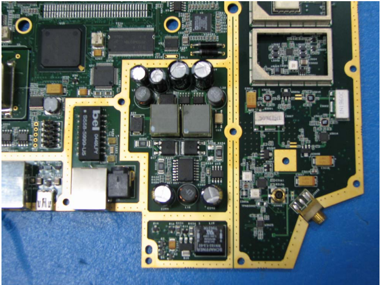
IP Access nanoBTS Top View – Lower Right
