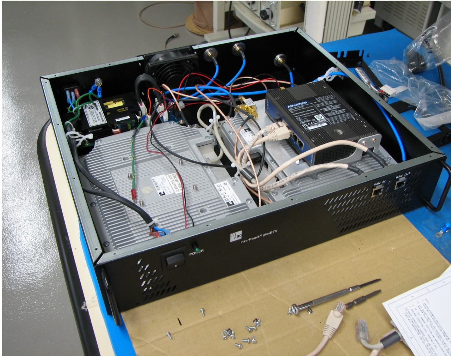
InterReach® picoBTS Top View / Cover Removed
