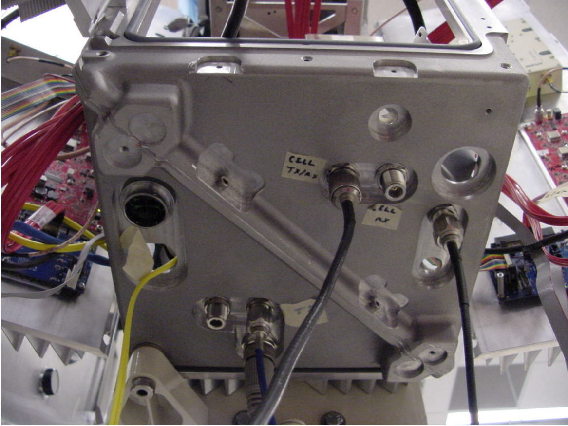
FlexWave™ URH Remote Unit Bottom View
