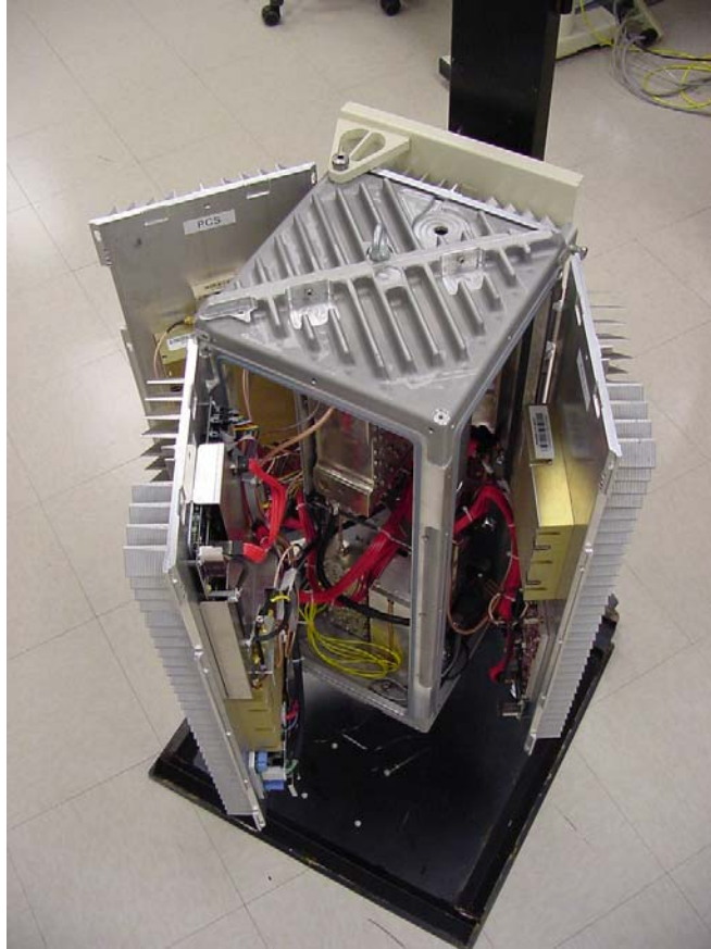
FlexWave™ URH Remote Unit Open Top View
